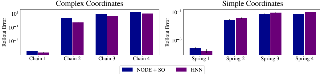
Figure 5: Left: Log rollout error for NODEs with second order bias and HNNs trained chain pendulums, where the analytic form of the Hamiltonian is simpler than the vector field. Right: Mechanic-sNNs and HNNs trained on spring pendulums, which have Hamiltonians and vector fields of similar complexity. HNNs outperform NODE with second order bias on systems that use non-Cartesian coordinates. Error bars show standard error across 5 seeds.
