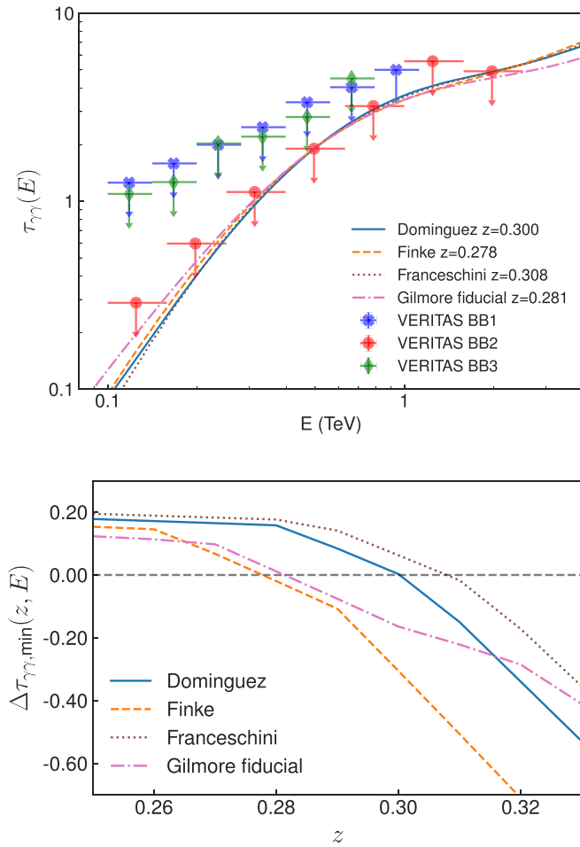
Figure 10. Top: the optical depth \tau_{\gamma}(E) of the gamma rays due to \gamma\gamma pair absorption induced by EBL photons. The blue filled crosses, the red filled circles, and the green filled diamonds show the 95% upper limits derived from VERITAS observations during periods BB1, BB2, and BB3, respectively. The optical depths \tau_{\gamma}(z, E) from four EBL models, Domínguez et al. (2011; blue solid line), Finke et al. (2010; orange dashed line), Franceschini et al. (2008; copper dotted line), and Gilmore et al. (2012; pink dashed-dotted line), evaluated at the maximum redshift allowed by the 95% upper limits are also shown. Bottom: the minimum difference between the 95% upper limits on the EBL-induced pair absorption optical depth \tau_{\gamma}(E) calculated from VERITAS data and the optical depth \tau_{\gamma}(z, E) calculated from EBL models as a function of redshift.
