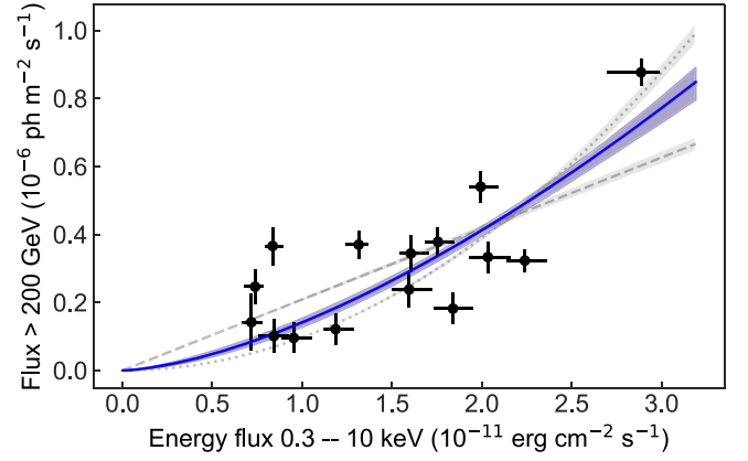
Figure 7. Scatter plot to investigate the correlation between the TeV gamma-ray flux and the X-ray energy flux. The flux measurements in the two bands were performed on the same nights. The gray dashed and dotted lines show the best linear and quadratic fits, respectively. The solid blue line shows the best power-law fit.
