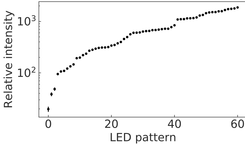
Fig 21 Relative intensity levels for several combinations of flasher LEDs measured in the laboratory. The absolute scale of the relative intensity corresponds to the approximate number of photoelectrons per pixel expected in the camera running on the telescope, accounting for pixel geometry and estimated photon detection efficiency. A selection of patterns were chosen which combine one or more Flasher LEDs. The intensity of these patterns were measured. Here the patterns have been ordered according to their intensity with 1 being the lowest and 60 being the highest.
