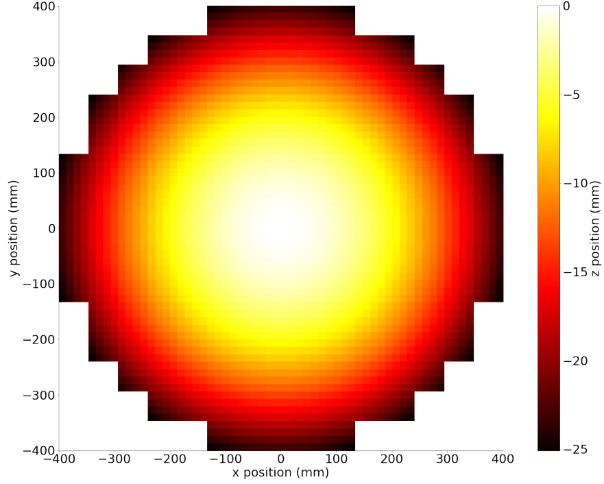
Fig 14 Camera Focal Plane. Colormap of the position of each trigger pixel in the camera. This plot is from the front perspective of the camera with the positive z axis toward the secondary mirror. The z-position of each quadrant is determined by shims placed between the SiPMs and the copper post. Trigger pixels within a quadrant are fixed at unique z-positions in relation to the quadrant. The final product is an approximation of a smoothly varying convex surface.
