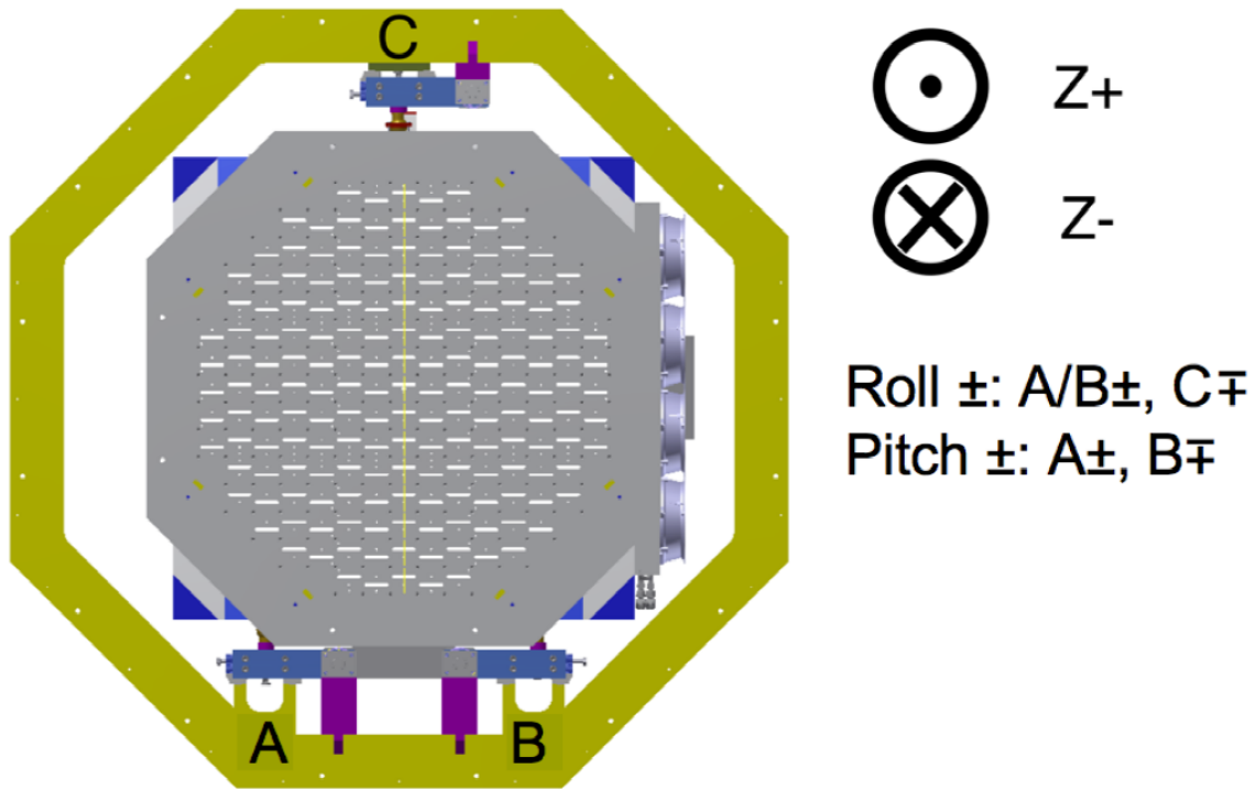
Fig 5 Motor locations in the pSCT camera as shown from the front. The yellow octagon is the outer structure of the camera and is connected with bolts to the telescope. The inner structure is movable via the three motors labeled A, B and C. Motion of the camera is described with a right-hand coordinate system with the z-direction labeled above along the optical axis of the telescope. z-motion of the camera requires that all motors move in unison. Pitch (rotation about the y axis) requires motors A and B moving in opposite directions. Roll (rotation about the x axis) requires motors A and B moving together and motor C moving in the opposite direction.
