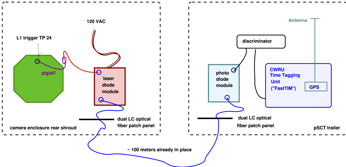
Fig 17 Conceptual schematic of the stand-alone camera event trigger time-tagging system for the pSCT. The Level-1 backplane trigger output is used to trigger a pulsed laser diode located at the back of the telescope. The laser pulse propagates via fiber optic cable to a photodiode detector which generates a GPS time-stamp accurate to better than 5 ns.
