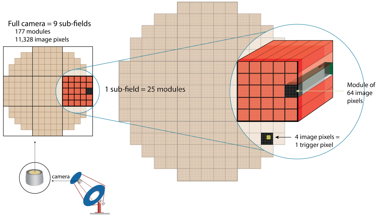
Fig 2 The pSCT camera has a hierarchical design. The full camera is comprised of 9 sectors, each of which can hold up to 25 camera modules (see Section 3). The sectors in each corner of the camera are equipped with fewer modules so that the entire camera has 177 modules. Each module has 64 image pixels so that the full camera will have 11,328 pixels. The current pSCT camera has only the center sector populated with modules.
