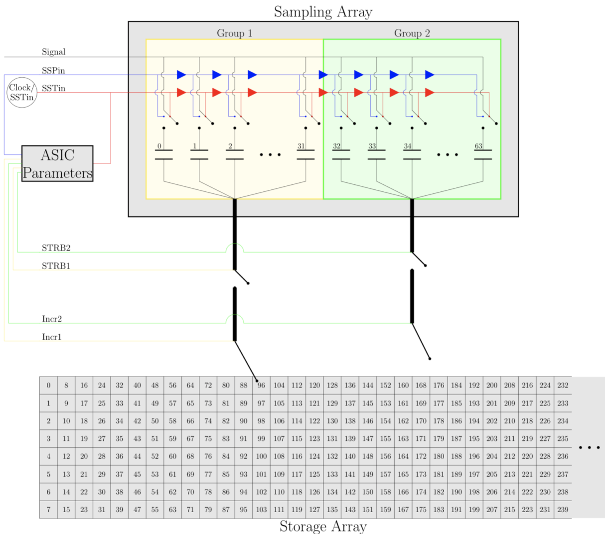
Fig 30 ASIC Diagram including ASIC Inputs, Sampling Array, and Storage Array and how they connect. The triangles on the SSTin and SSPin lines are 1 ns delay elements. When a signal hits a delay element it is delayed by 1 ns for each element. Notice there are no delay elements on the Signal line. The incoming signal hits all the capacitors simultaneously. The Incr1 and Incr2 switches can connect to any Storage Array block, though the mechanism is more complicated than depicted here.
