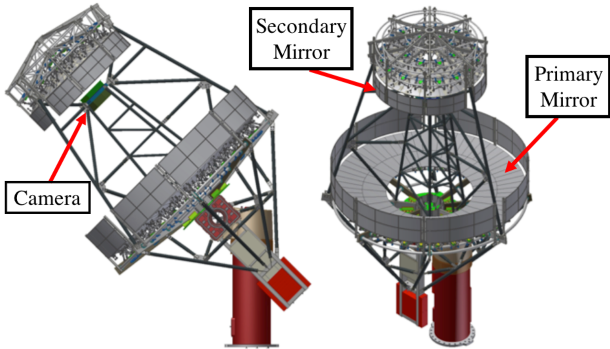
Fig 1 Artists rendition of the prototype Schwarzschild-Couder Telescope. Schwarzschild-Couder optics utilize two mirrors and a curved focal plane to achieve excellent resolution and sensitivity. The Primary (9.66 m) and Secondary (5.4 m) Mirrors are labeled above along with the location of the camera. Figure taken from. 4
