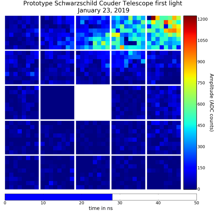
Fig 27 First light from the pSCT. First light and first shower candidates were achieved on January 23, 2019. This is a snapshot of a single event. The center module is blank because that position is temporarily occupied by an alignment calibration module. The module in the center left is dark because it failed to connect on this run.
