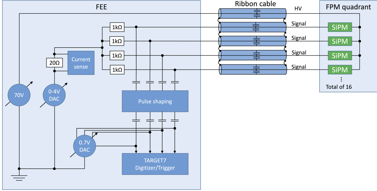
Fig 16 A block diagram of the signal chain between SiPM sensors of one FPM quadrant and a single TARGET7 readout chip (of four in one module). The 0 – 4 V DAC adjusts the bias voltage across groups of 4 SiPMs for differences in their breakdown voltage. The 0.7 V DAC provides a pedestal offset to the signals entering the digitizer chip.
