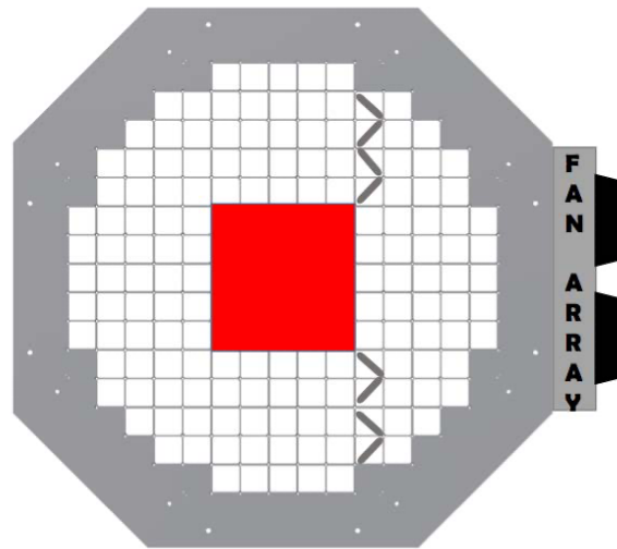
Fig 8 Air baffle orientation diagram. Baffles are long, rectangular aluminum pieces which are inserted into unused module slots at a 45° angle. The baffles are arranged in such a way that air from the fans is directed through the modules in the camera. These baffles will be removed for the camera upgrade to make room for the modules of the fully populated focal plane. The camera upgrade will also include additional fans in order to cool the increased number of modules.
