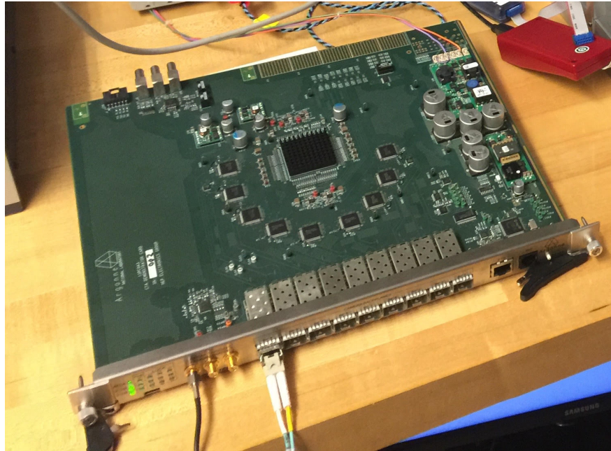
Fig 36 Photo of the demonstrator Distributed Intelligent Array Trigger (DIAT) on a laboratory test stand, connected to the pSCT camera backplane. The DIAT is a single-board custom-designed module for time-tagging, timing synchronization, hit pattern processing and cross-triggering. Fiber optic ports on the front panel connect to up to nine SCT backplanes for the full-sized camera.
