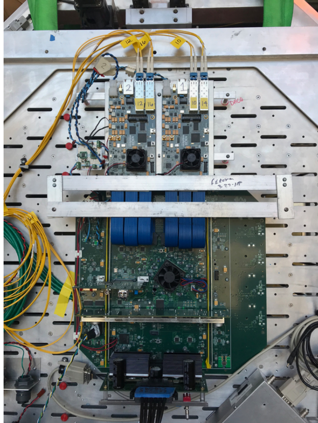
Fig 35 Photo of the backplane. The back bulkhead has two holes per module, one long slit for the module backplane connector and one for the module securing screw. The backplane is mounted onto this back bulkhead. Each module connects to the backplane through a backplane connector and is secured with a screw running through the backplane, bulkhead and module. On top of the backplane are mounted two DACQ boards (top), one power board (middle) and two power connectors (bottom). The DACQ boards have two fiber cables each (yellow) leading to the network switch. The green cables allow a central alignment device, which can be installed instead of the central module, to connect to a positioner. This device is used to align the camera and optics. The Raspberry Pi is in an aluminum box in the lower right hand corner and is connected to the backplane via an SPI link through a D-shell connector. The fans are connected to the backplane via a small board in the upper left hand corner.
