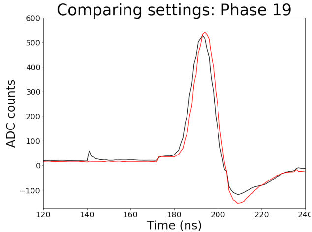
Fig 32 In order to compare the original ASIC settings (shown in black) to the optimized settings (shown in red and listed in table 1), data was taken using an LED flasher with an asynchronous trigger provided by an external signal generator. The data was pedestal subtracted and averaged, once for the previous settings and once for the new settings. Because, the location of the pulse in relation to the block boundary (called the “phase”) determines where the pre-pulse is located in the waveform the two settings were compared individually for every phase. The figure on the right shows the difference between the previous and new settings for a single phase. It is clear that the New ASIC Settings reduce the pre-pulse. Similar results are found for all phases.
