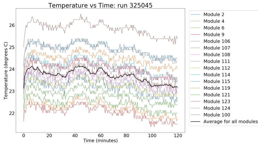
Fig 10 Temperature vs time for a two hour run taken onsite during the summer of 2018 (prior to installation of the Peltier coolers and control). The ambient temperature over the course of the run was 22.8 C - 23.9 C. Module temperature is recorded on the module's front end electronics. The temperature of each individual FEE is constant to within 1° over the full two hour period. Typical data runs last one hour meaning that individual modules do not experience significant changes in temperature within a single run. The spread of temperatures across modules is due to their physical position in the camera and is consistent over time. Additionally, Each module has an independent lookup table for temperature-dependent variables to account for the 4° spread between modules.
