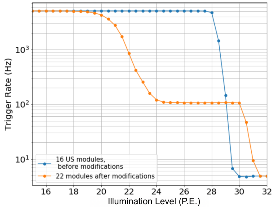
Fig 24 Trigger noise reduction. Prior to noise reduction steps the trigger noise was high enough that it saturated the trigger system. After these noise-reducing modifications the trigger rate was reduced to 22 PE for a 1 kHz trigger rate. 4
