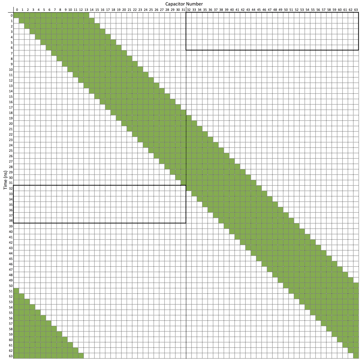
Fig 31 Holding/Tracking diagram for the optimized ASIC settings. Capacitors are labeled on the top of the diagram and as we move down the figure time progresses in steps of 1 ns. The state of each capacitor is given by the color. Green means the capacitor is in tracking mode while white means it is in holding mode. The thick black boxes indicate the duration of the STRB for each group of capacitors.
