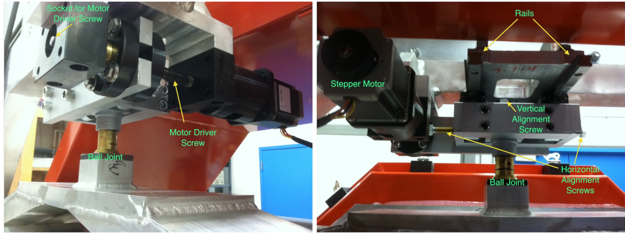
Fig 33 Photo of Motor assembly C, located at the top of the camera. Labeled are the ball joint, motor driver screw, rails, vertical and horizontal alignment screws, and the stepper motor.
