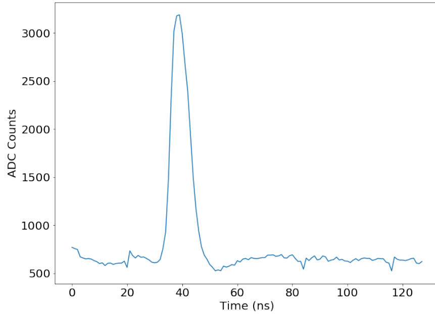
Fig 19 Flasher pulse taken onsite using a flasher on the optical table with the potentiometer set at 6 k \Omega . No pedestal or baseline subtraction has been applied.
