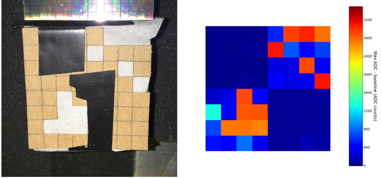
Fig 23 The face of a single module FEE was first covered with a tissue (which allows light to pass through) and then with a cardboard mask. The mask was affixed to the FEE with black electrical tape. An LED was flashed on the prepared FEE. The left shows a picture of the physical setup of the module. The right shows the heatmap of average waveform height in different channels. Some cross-talk exists between adjacent pixels in the same quadrant. However, it is clear that the ASIC channels are connected to the correct Pixel IDs, as those pixels exposed to LED pulses have significantly larger average waveform heights.
