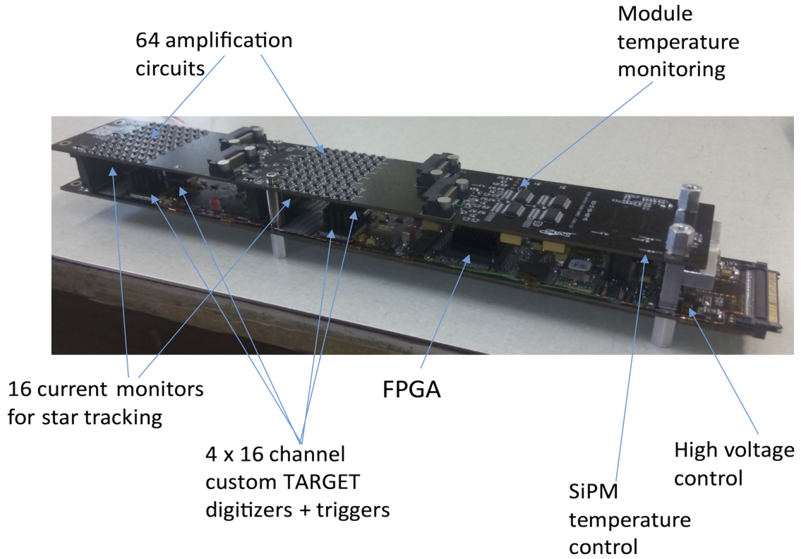
Fig 15 The pSCT front-end electronics. The auxiliary board is stacked on top of the primary board and they are connected with high-speed connectors. The primary board connector on the right-hand side connects the module to a backplane when it is mounted in the camera.
