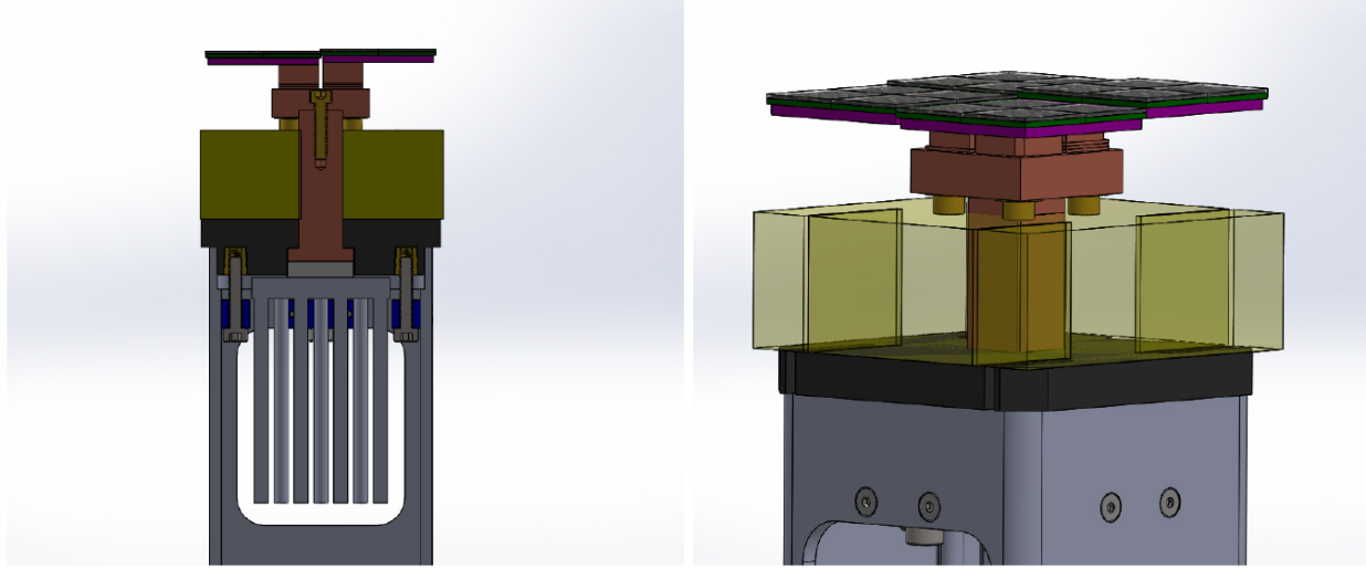
Fig 9 Two perspectives of an FPM. Each FPM is divided into four quadrants. Each quadrant is composed of 16 image pixels and has a z position achieved by placing shims between the copper post and the copper block on the bottom of the PCB for each quadrant. Yellow insulating foam surrounds the copper post which attaches the light sensors to a Peltier element. On the opposite side of the Peltier element is a heat sink.
