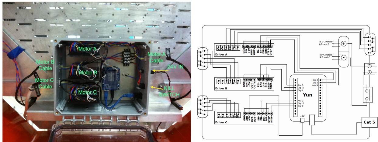
Fig 34 Photo (left) and circuit diagram (right) of the motor electronics box located in the back of the camera. This box includes an Arduino and three motors which control the movement of each stepper motor.
