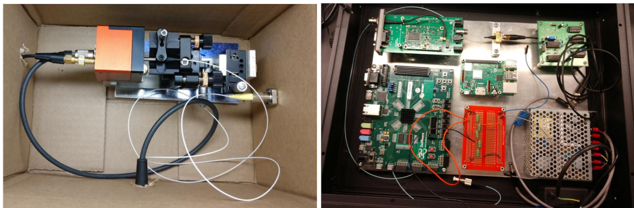
Fig 37 Photos showing main components of the stand-alone timing system: the laser-diode module which is installed near the telescope camera backplane (left) and the photo-diode and GPS timing module which is installed in the pSCT trailer (right).
