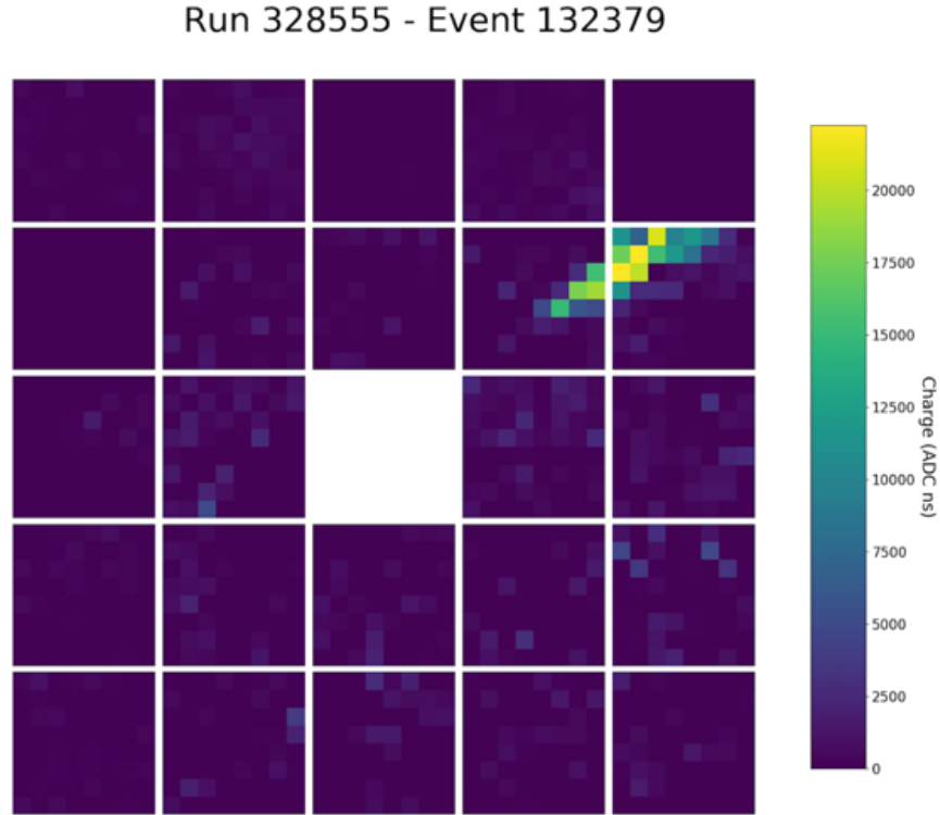
Fig 28 First confirmed gamma-ray-like event recorded by the pSCT. This event was taken on January 17, 2020 with simultaneous observation with VERITAS. This event was confirmed as a gamma-ray via timing coincidence with simultaneous VERITAS observation.
