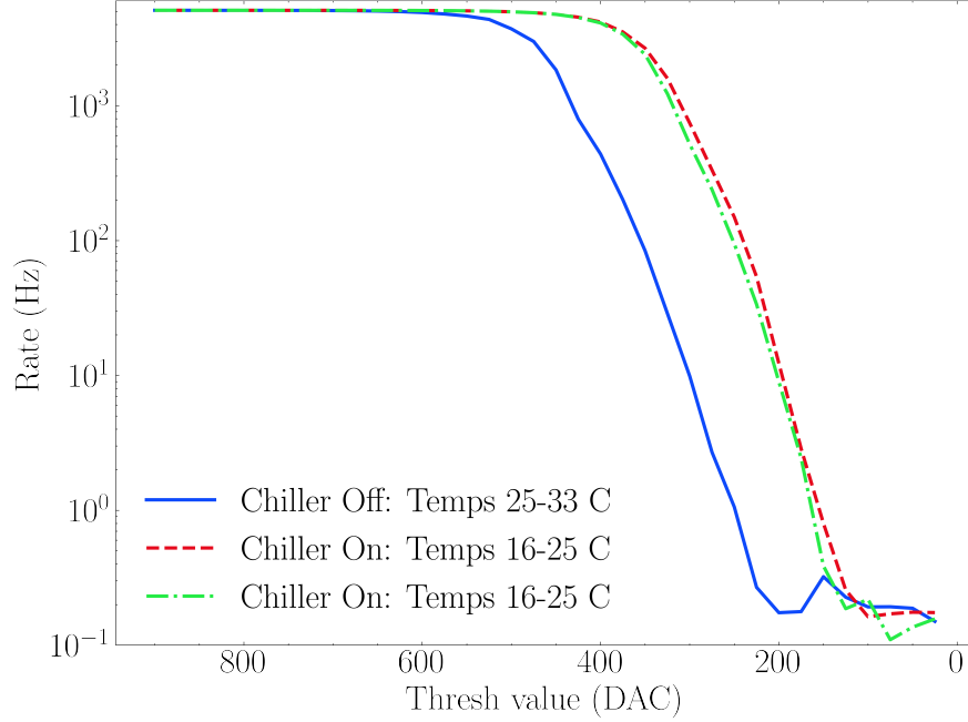
Fig 26 Rate scans included all modules and were taken with the shutter open on the same night so that ambient conditions were the same. One rate scan was taken with the chiller off, resulting in warmer average module temperatures. Two rate scans were taken with the Chiller on resulting in colder temperatures. Rate scans with a lower temperature are shifted to lower Thresh values (corresponding to a higher physical threshold).
