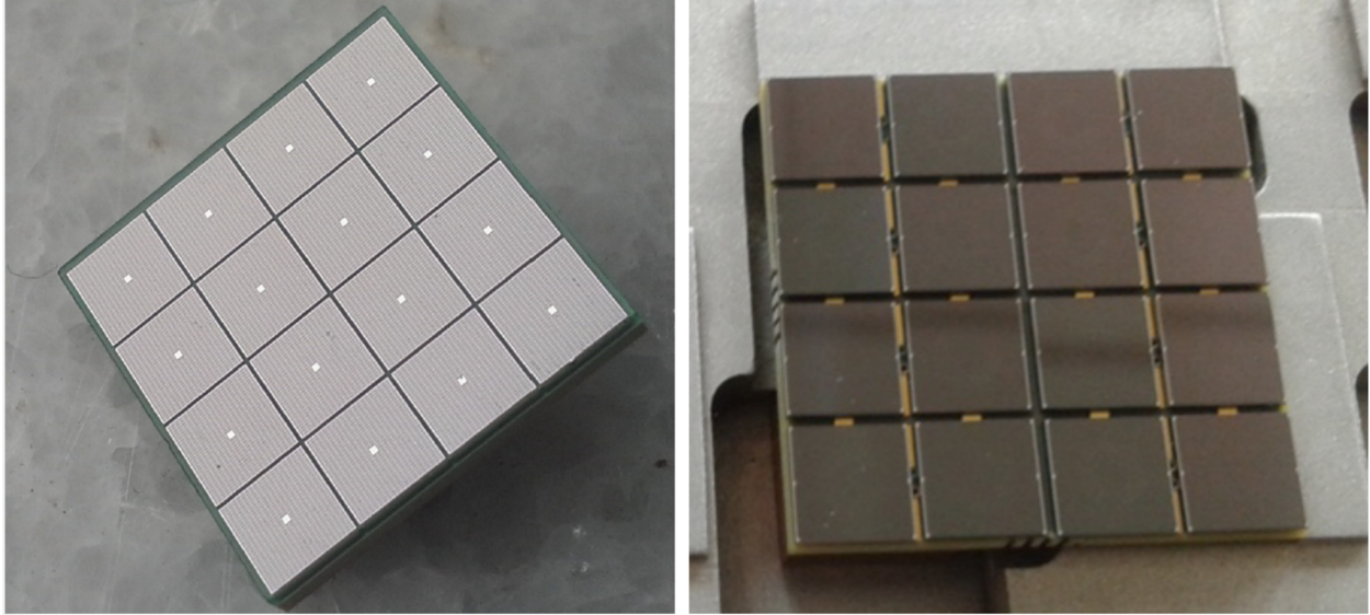
Fig 12 On the left is a photo of a Hamamatsu MPPC S12642-0404PA-50(X) sensor used in the pSCT camera. Shown is a single tile as delivered by the manufacturer. Each tile has 16 3x3 mm SiPMs which are grouped into four 6x6 mm image pixels. Each tile corresponds to one Trigger Pixel and A single FPM uses 16 of these tiles. 13 A single Hamamatsu tile measures 13x13 mm. On the right is a photo of an FBK sensor used in the pSCT camera. Shown is a single tile. Each tile has 16 6x6 mm SiPMs each of which correspond to a single image pixel. Each tile corresponds to 4 Trigger Pixels and a single FPM uses 4 of these tiles. A single FPM tile measures 26x26 mm
