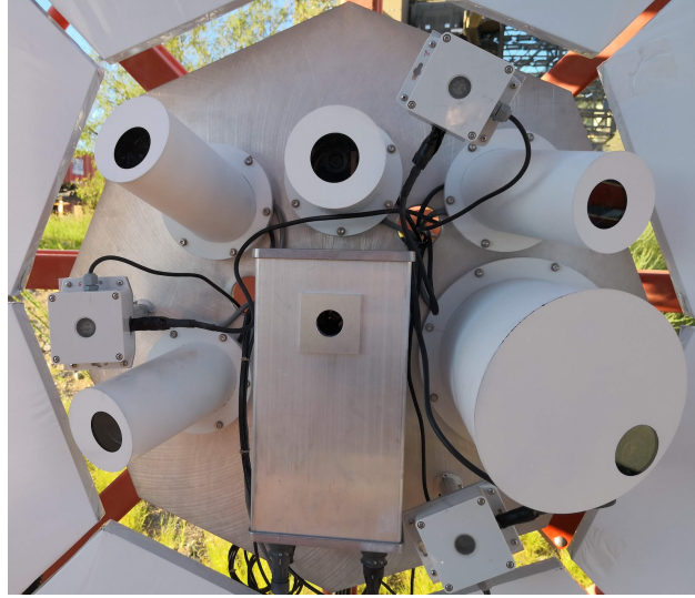
Fig 18 Optical Table located at the center of the secondary reflector. The flashers are the square object mounted along the exterior. From top to bottom the flashers have potentiometer settings 2.5 k \Omega , 1.8 k \Omega , 4 k \Omega . The flasher set to 4 k \Omega is also equipped with a 10% neutral density filter.
