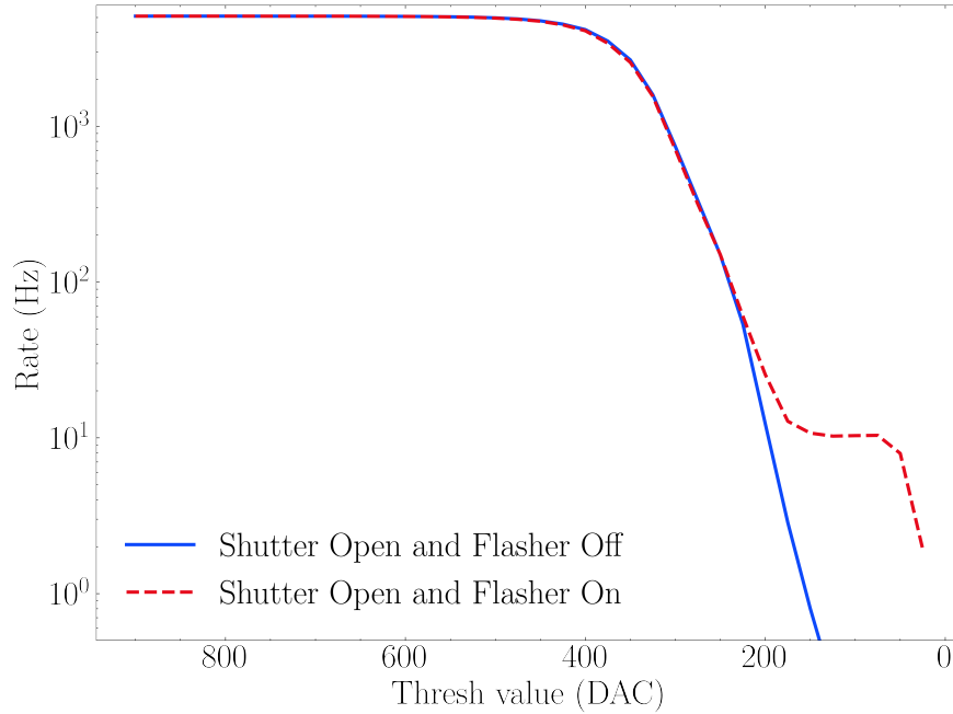
Fig 25 Rate scans with flasher on and off. Rate scans included all modules and were taken under typical operating conditions in the same night. The rate scan taken with the flasher on shows a clear plateau at 10 Hz (the same rate at which the flasher was run).
