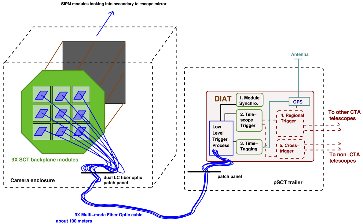
Fig 29 Conceptual schematic of the operation of the Distributed Intelligent Array Trigger (DIAT) module (right) in relation to the full SCT camera with nine backplanes (left). Low-level trigger and timing messages from individual detector modules (FEE) are collected and relayed with timing information by each of nine backplane modules via fiber optic lines. The DIAT module (located within the telescope trailer) has five functions: (1) synchronization of detector modules, (2) telescope Triggers, (3) GPS time-tagging, (4) regional Triggers (via shared hit-patterns) and (5) cross-triggers with other telescopes in CTA. For the pSCT, the DIAT demonstrator module provides functions (1)–(3) as required for a single backplane.
