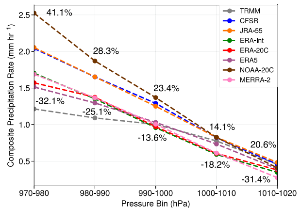
FIG. 8. Composite mean precipitation rate and binned MSLP (10-hPa width) for IBTrACS-derived TC precipitation in reanalyses and TRMM (1998–2010). Percentages shown are the maximum and minimum percent error from the mean across the seven reanalyses in each intensity bin as an indication of the reanalysis spread.
