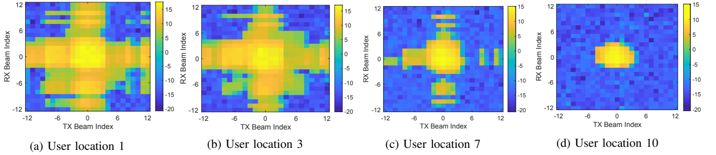
Fig. 5: SNR heatmaps for all beam pair combinations for user location indices 1, 3, 7 and 10 in the corridor.
