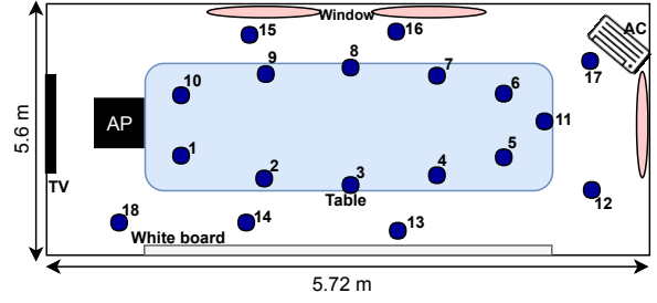
Fig. 11: Experimental floor plan used for measurement of data using WARP-60 testbed.
