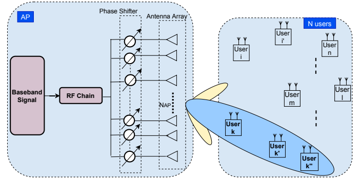
Fig. 1: AP with single RF chain system supporting multiple users
