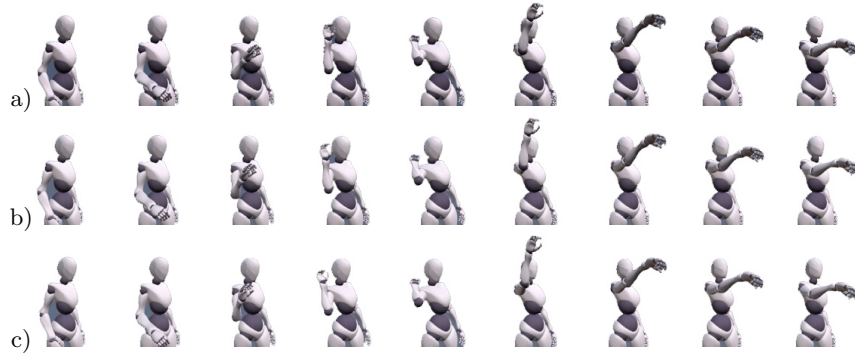
Fig. 3: Metaphoric gesture: LinEuler a), Slerp b), and Squad c).
