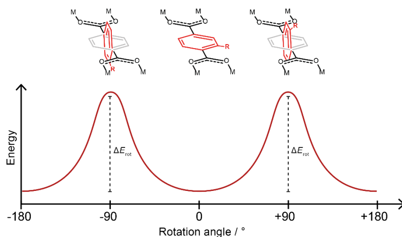
Chart 1. Energy profile of a terephthalate rotor linker.
