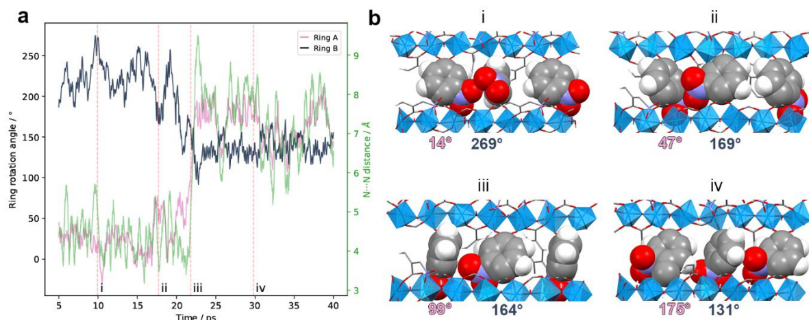
Figure 5. Cooperative rotation in NO 2 -MIL-53(Al). a , Rotation angle traces of two neighboring rings in a 2x1x1 cell MD simulation at 700 K. Correlated motion is observed, with simultaneous angle changes in opposite directions (i,ii,iii), when nitro groups are in proximity (N...N distance ca. 4 Å). b , Selected snapshots (i-iv) of linker pair conformation during a coupled rotation. As ring A rotates in the positive direction, ring B reaches the space originally occupied by ring A.
