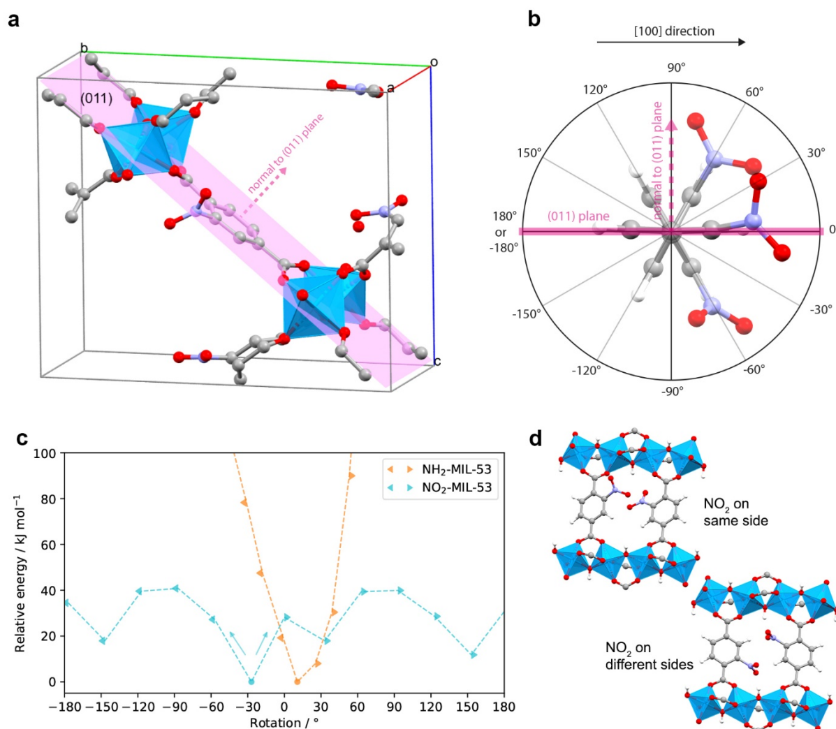
Figure 2. Effect of linker rotation on the potential energy as studied by DFT. a, Unit cell of NO 2 -MIL-53(Al) with central linker in 0° rotation with respect to (011) plane (pink); hydrogens omitted for clarity. b, Rotation angle is defined as the angle between benzene ring plane and (011) plane, taking 0° as the conformation with the functional group pointing in the positive [100] direction. The sign of the angle is assigned based on the direction normal of the reference plane. c, Potential energy profiles for the rotation of one linker in a NH 2 -MIL-53(Al) and NO 2 -MIL-53(Al) unit cell. The direction of rotation is indicated
