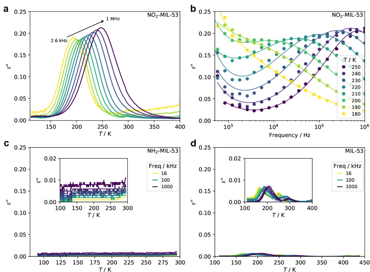
Figure 3. Dielectric spectra of the three systems. a,b , Imaginary part ( \epsilon'' ) of \epsilon^* for NO 2 -MIL-53(Al) with respect temperature to (a) and frequency (b) . The latter includes the fitted Cole-Cole model as continuous lines. c,d , Temperature dependence of \epsilon'' for NH 2 -MIL-53(Al) (c) and MIL-53(Al) (d) .
