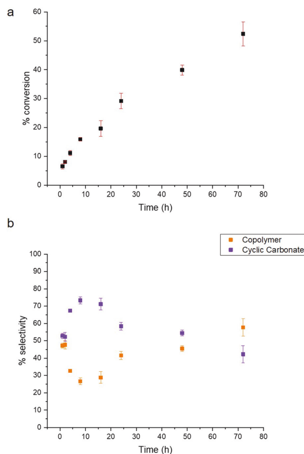
Fig. 4 (a) % conversion versus time of copolymerisation of xylose oxetane with CO 2 (b) % selectivity of the cyclic carbonate and copolymer as a function of time during the copolymerisation.
