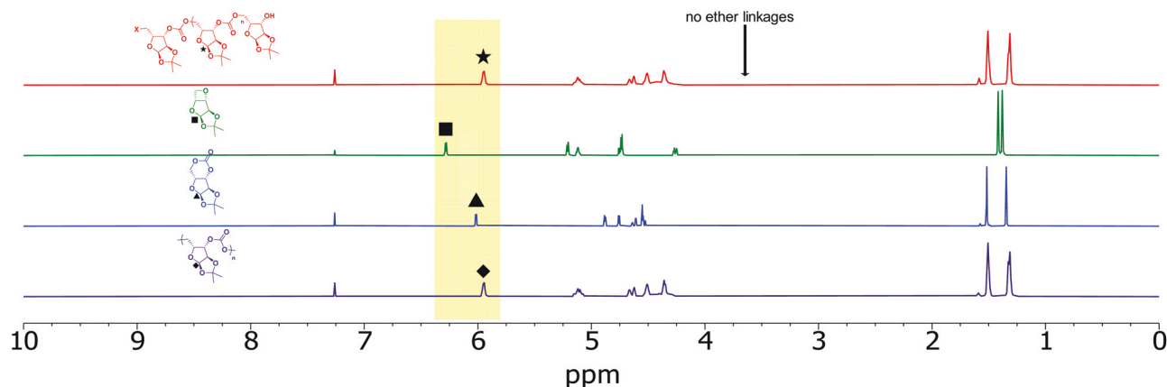
Fig. 2 ^1\text{H} NMR spectra of poly(1,2- O -isopropylidene- \alpha -D-xylofuranose carbonate) 5 from ROCOP (red trace), 3,5-anhydro-1,2- O -isopropylidene- \alpha -D-xylofuranose ( 4 , green trace), 1,2- O -isopropylidene- \alpha -D-xylofuranose carbonate ( 6 , blue trace), and poly(1,2- O -isopropylidene- \alpha -D-xylofuranose carbonate) 7 from organocatalysed ROP (purple trace), where the chemical shift of the anomeric position of each compound is located in the highlighted region.
