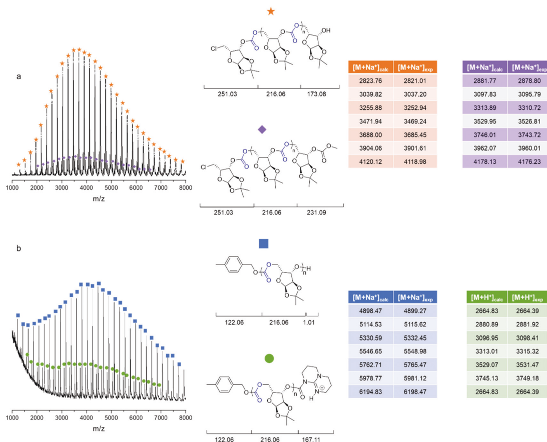
Fig. 3 MALDI-ToF spectra of (a) copolymer produced from ROCOP of \text{CO}_2 and xylose oxetane. (b) Polymer produced from TBD-catalysed ROP of 1,2- O -isopropylidene- \alpha -D-xylofuranose carbonate.
