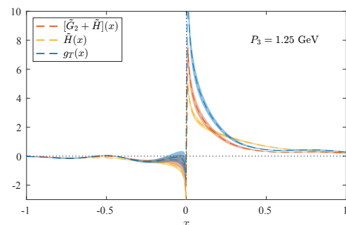
Figure 4: The matched GPD \tilde{G}_2(x) + \tilde{H}(x) compared to the purely twist-2 helicity GPD \tilde{H}(x) and the twist-3 PDF g_T(x) .
