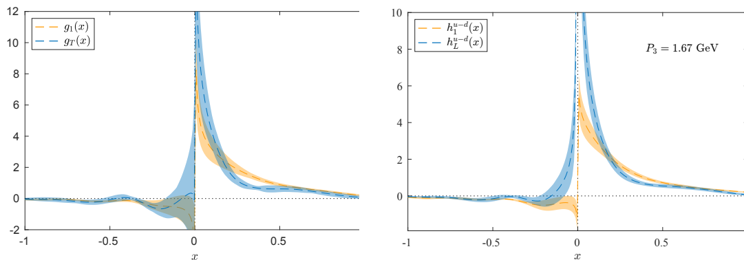
Figure 2: Comparison of the twist-3 PDFs with their twist-2 counterparts: g_T(x) vs. g_1(x) (left) and h_L(x) vs. h_1(x) (right).
