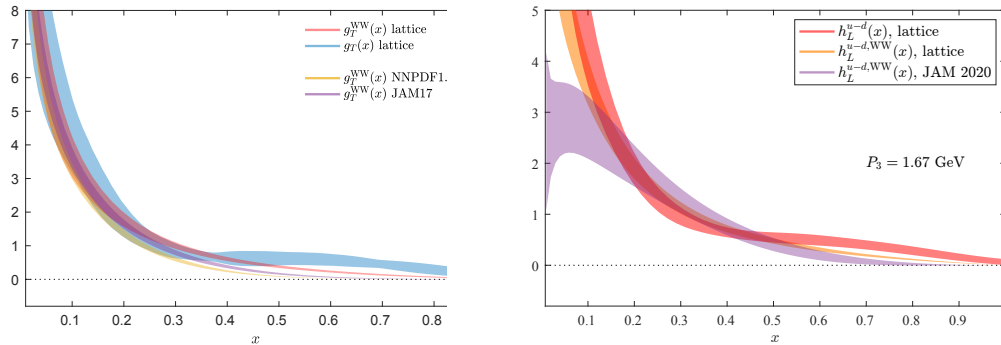
Figure 3: Test of the WW approximation for g_T(x) (left) and h_L(x) (right).
