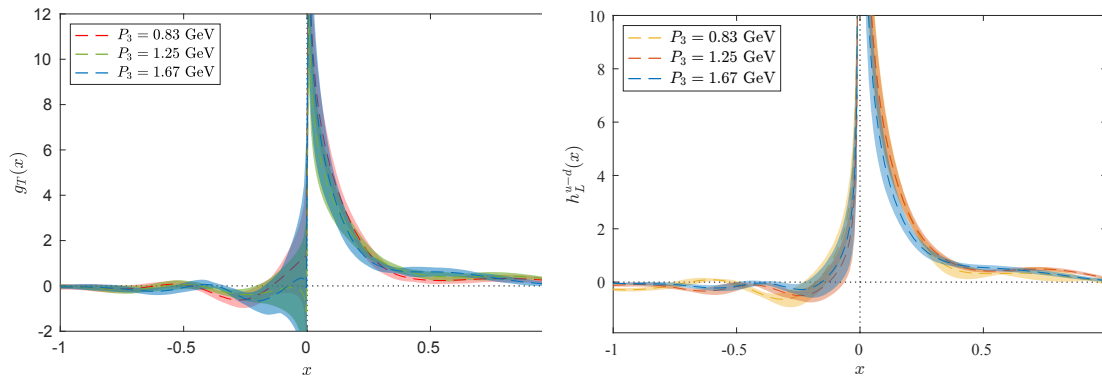
Figure 1: Nucleon momentum dependence of g_T(x) (left) and h_L(x) (right).
