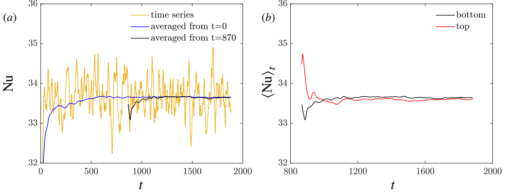
Figure 2: (a) Time series and running average of the Nusselt number on the bottom wall. (b) Running average of the Nusselt number on both the bottom and top walls. The plots correspond to the case \Phi = 20\% and d_p^* = 1/15 .
