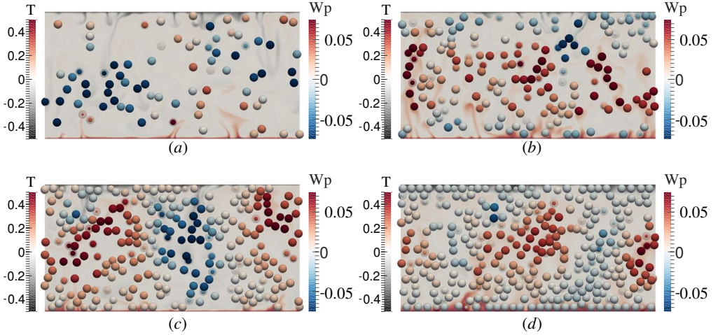
Figure 3: Snapshots of the temperature field along with the particle locations in a wall-normal y - z plane. The particles are coloured based on their vertical velocity w . (a) \Phi = 10\% , (b) \Phi = 20\% , (c) \Phi = 30\% , and (d) \Phi = 40\% . In all the cases, d_p^* = 1/15 . Since the contour plane is partially transparent, the particles with centers located behind the plane appear to have a halo around them.
