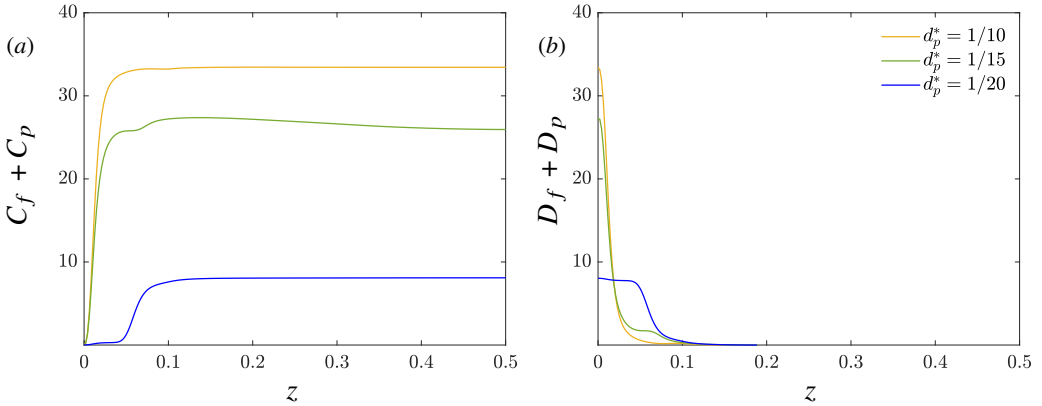
Figure 22: Convective and diffusive contributions to the total heat transfer for different dimensionless particle diameters. (a) Convection by both the fluid and particle velocity fluctuations, and (b) molecular diffusion in both phases.
