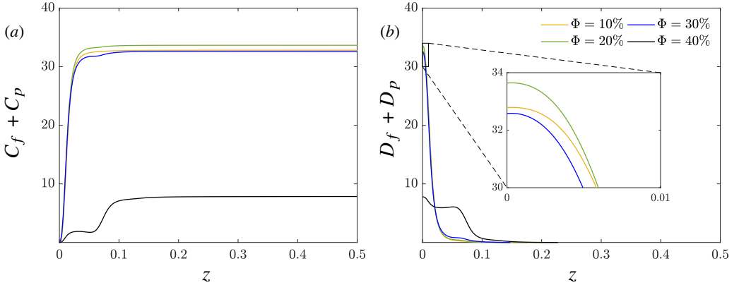
Figure 16: Convective and diffusive contributions to the total heat transfer for different particle volume fractions. (a) Convection by both the fluid and particle velocity fluctuations, and (b) molecular diffusion in both phases. In all the cases, d_p^*=1/15 .
