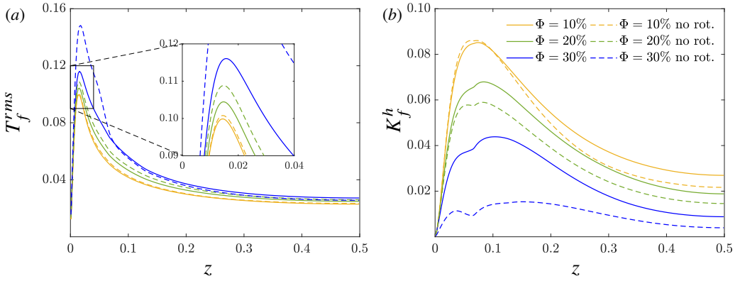
Figure 13: Comparison between simulations where particle rotation is allowed and when it is not allowed. (a) Temperature rms of the fluid phase, and (b) horizontal contribution of the kinetic energy per unit mass of the fluid. In all the cases, d_p^* = 1/15 .
