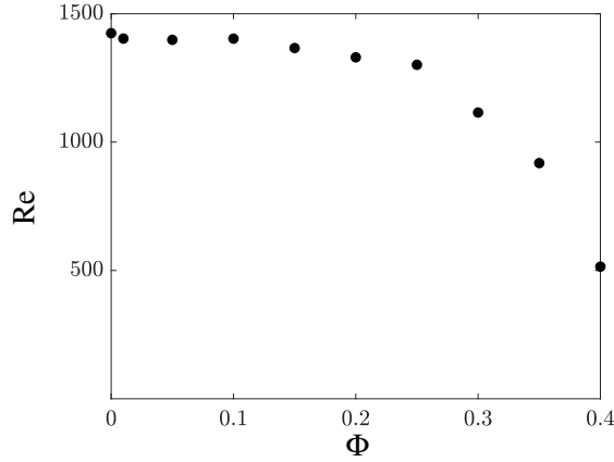
Figure 10: Reynolds number based on the maximum rms value of the fluid vertical velocity, Re = Lw_f^{rms}/\nu , as a function of the particle volume fraction, for d_p^* = 1/15 .
