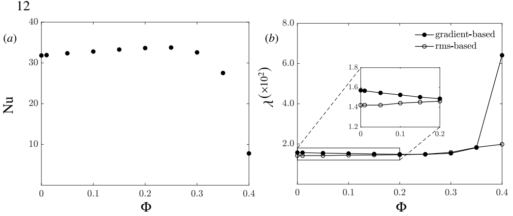
Figure 6: (a) Nusselt number and (b) thermal boundary layer thickness as a function of the particle volume fraction, for d_p^*=1/15 . The boundary layer thickness based on the gradient is defined in equation (3.1) and the rms-based definition given in equation (3.2). Both quantities are calculated by averaging the relevant quantities at the bottom and top walls.
