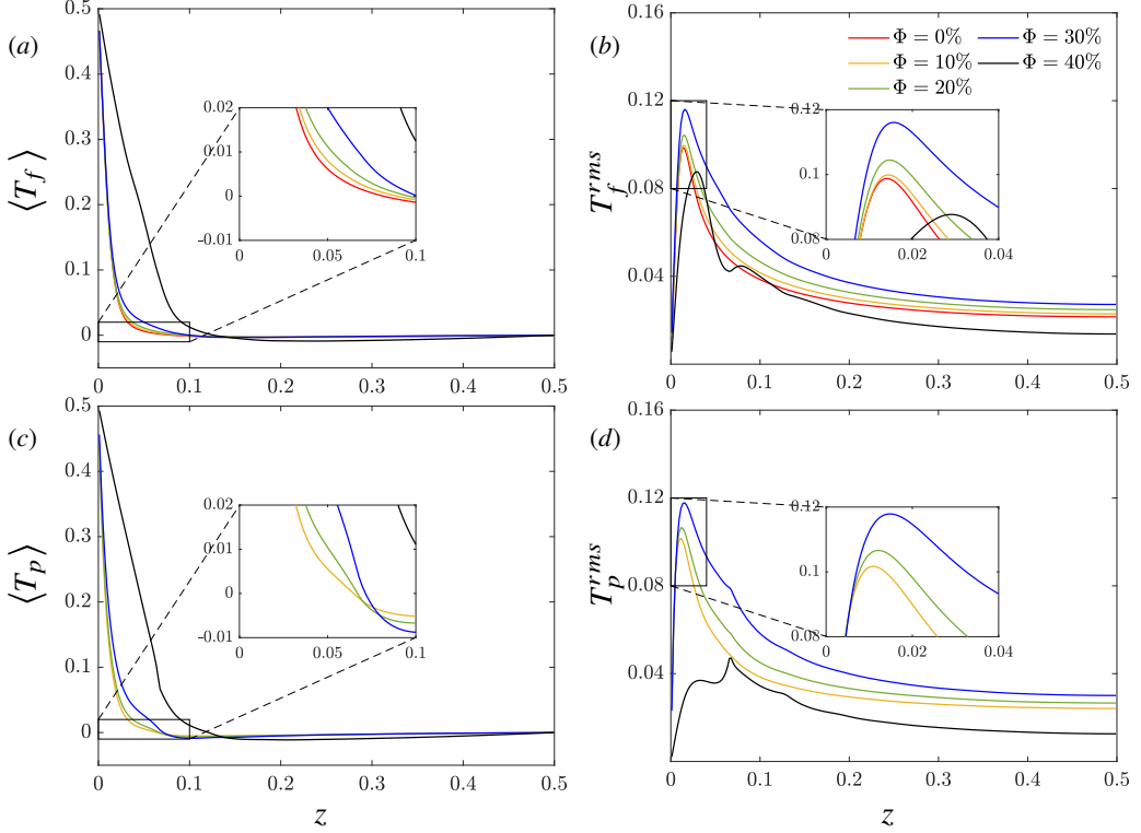
Figure 8: Wall-normal profiles of the temperature statistics for different values of the particle volume fraction. (a) Mean fluid temperature, (b) rms of the fluid temperature, (c) average particle temperature and (d) rms values of the particle temperature. In all the cases, d_p^* = 1/15 .
