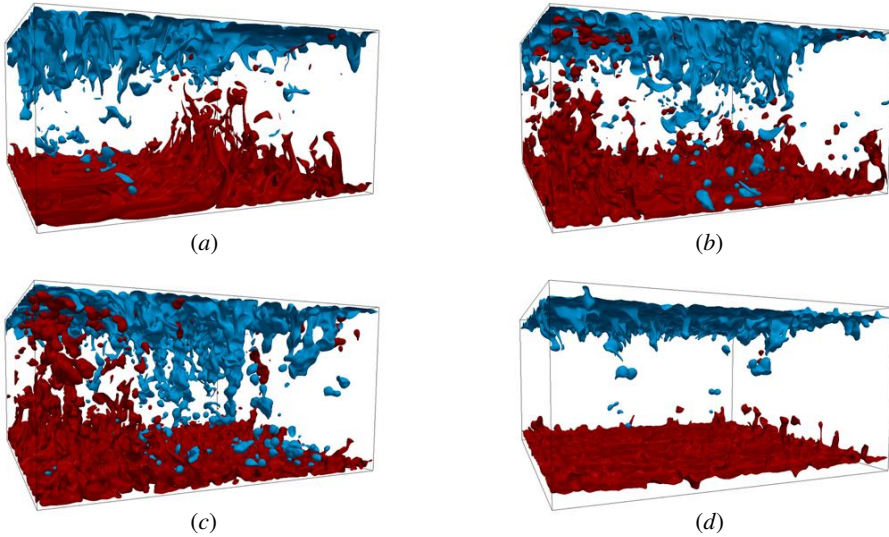
Figure 5: Snapshots of temperature isosurfaces for (a) \Phi = 10\% , (b) \Phi = 20\% , (c) \Phi = 30\% , and (d) \Phi = 40\% . In all the cases, d_p^* = 1/15 . Red colour corresponds to T = 0.1 and blue colour corresponds to T = -0.1 .
