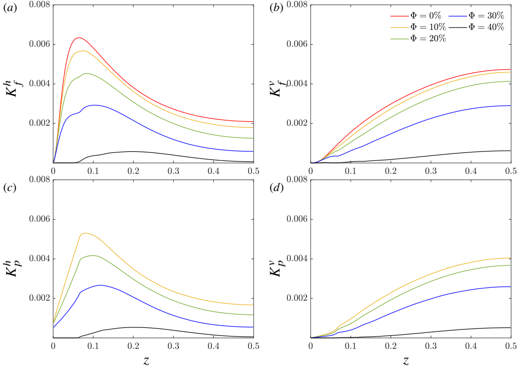
Figure 9: Components of the average kinetic energy per unit mass, derived from the velocity rms, as a function of the vertical direction for the different particle volume fractions indicated. (a) Horizontal and, (b) vertical contribution of the fluid, see equation (3.3); (c) horizontal and, (d) vertical contribution from the particles, defined in equation (3.4). In all the cases, d_p^* = 1/15 .
