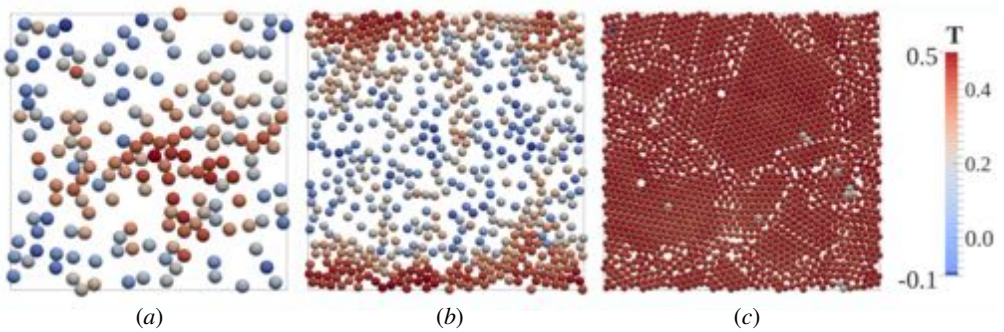
Figure 19: Snapshots of the first particle layer next to the bottom wall ( x - y plane). The particles are coloured based on their temperature. (a) d_p^* = 1/10 , (b) d_p^* = 1/15 , and (c) d_p^* = 1/20 . In all the cases, \Phi = 35\% .
