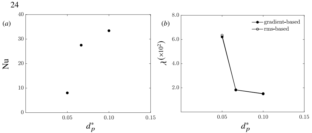
Figure 18: (a) Nusselt number and (b) thermal boundary layer thickness as a function of the dimensionless particle diameter, for \Phi = 35\% . The boundary layer thickness based on the gradient is defined in equation (3.1) and the rms-based definition given in equation (3.2). Both quantities are calculated by averaging the relevant quantities at the bottom and top walls.
