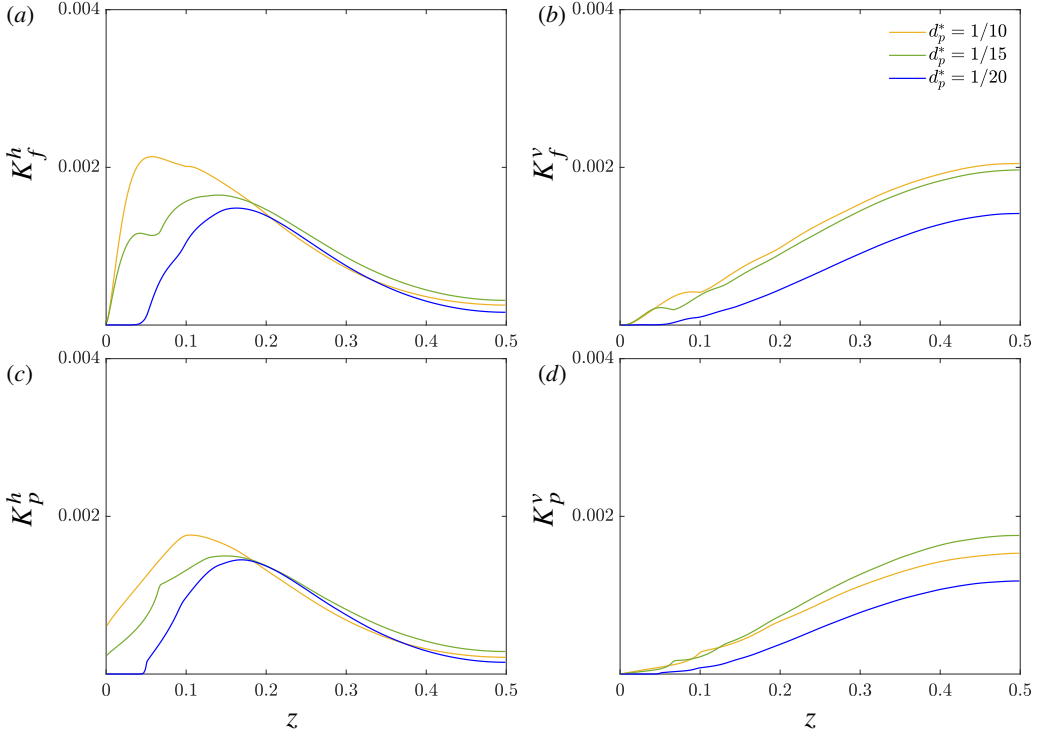
Figure 21: Components of the average kinetic energy per unit mass, derived from the velocity rms, as a function of the vertical direction for the different dimensionless particle diameters indicated. (a) Horizontal and, (b) vertical contribution of the fluid, see equation (3.3); (c) horizontal and, (d) vertical contribution from the particles, defined in equation (3.4).
