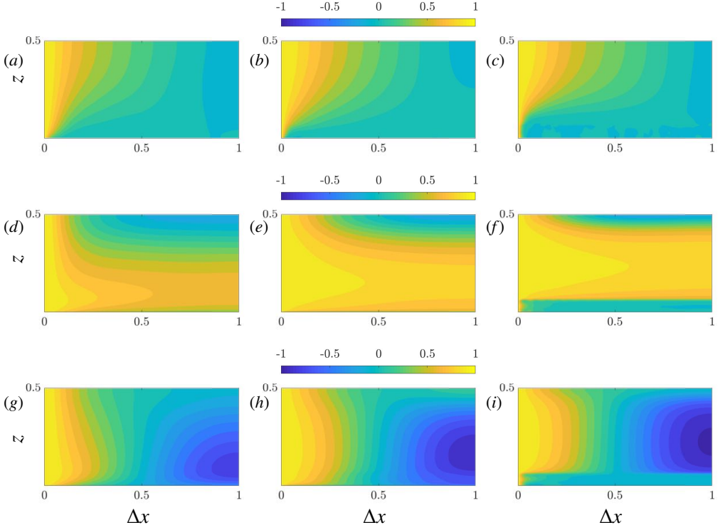
Figure 17: Contour plots of the two-point velocity correlations. Top row, (R^x_{ww} + R^y_{ww})/2 ; middle row, (R^x_{uu} + R^y_{vv})/2 ; and bottom row, (R^x_{vv} + R^y_{uu})/2 . Left column, \Phi = 0\% ; middle column, \Phi = 35\% ; and right column \Phi = 40\% . In all the cases, d_p^* = 1/15 . Since the x - and y -directions are homogeneous and the two point correlations are statistically equivalent in pairs, the results shown here are also valid if \Delta x is replaced with \Delta y in the x -axis of the figure.
