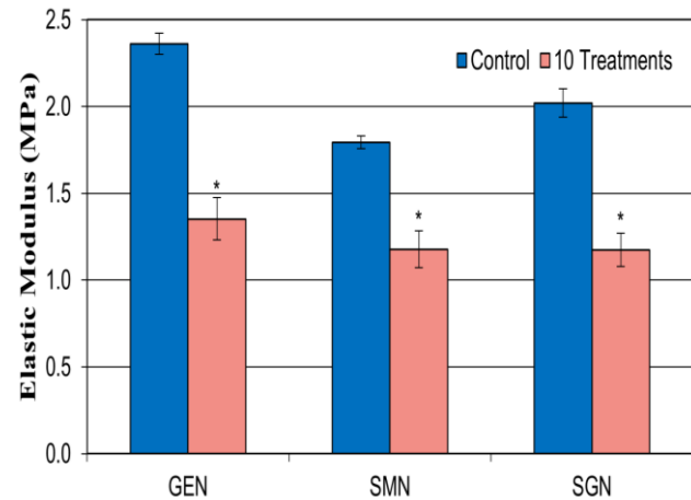
Fig. 4. Effect of 10 treatments of soap and water on nitrile gloves' elastic modulus.
