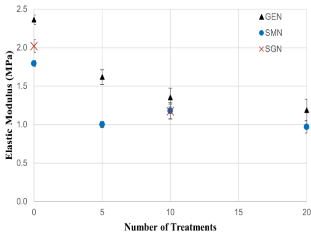
Fig. 5. Effect of the number of soap and water treatments on nitrile gloves' elastic modulus.
