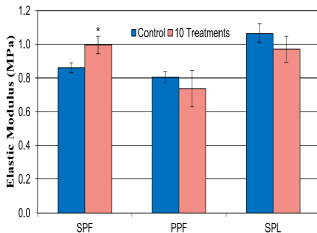
Fig. 6. Effect of 10 treatments of soap and water on latex gloves' elastic modulus.
