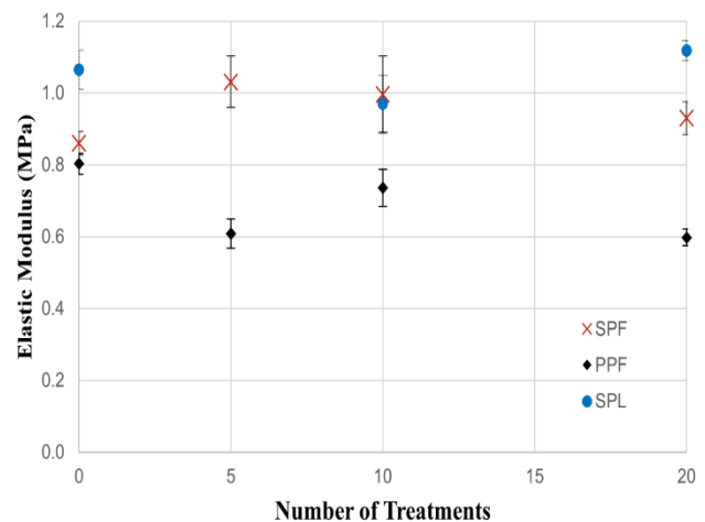
Fig. 7. Effect of the number of soap and water treatments on latex gloves' elastic modulus.
