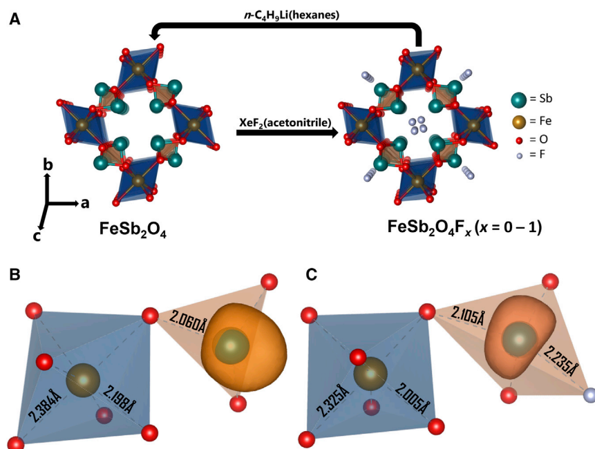
Figure 1. Reversible topochemical fluoride-ion insertion in \text{FeSb}_2\text{O}_4
