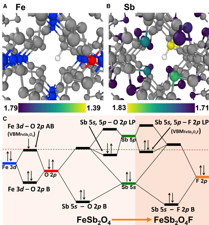
Figure 7. A molecular orbital perspective of electronic structure modulation of FeSb 2 O 4 with fluoridation
