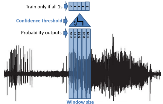
Figure 2: A windowing scheme, tuned using two hyperparameters, is implemented to only train the classifier once a series of high-confidence predictions are generated, allowing for a more robust model over time.
