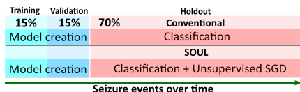
Figure 4: Dataset division between training, validation and holdout while preserving the time series nature of the data. SOUL enables unsupervised model updates during classification on the holdout set.
