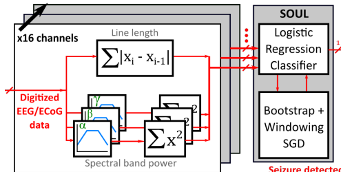
Figure 3: Seizure detection system implemented in this work. Line length and spectral band powers for each of the 16 channels are calculated in parallel which are then fed into SOUL for classification and model update.
