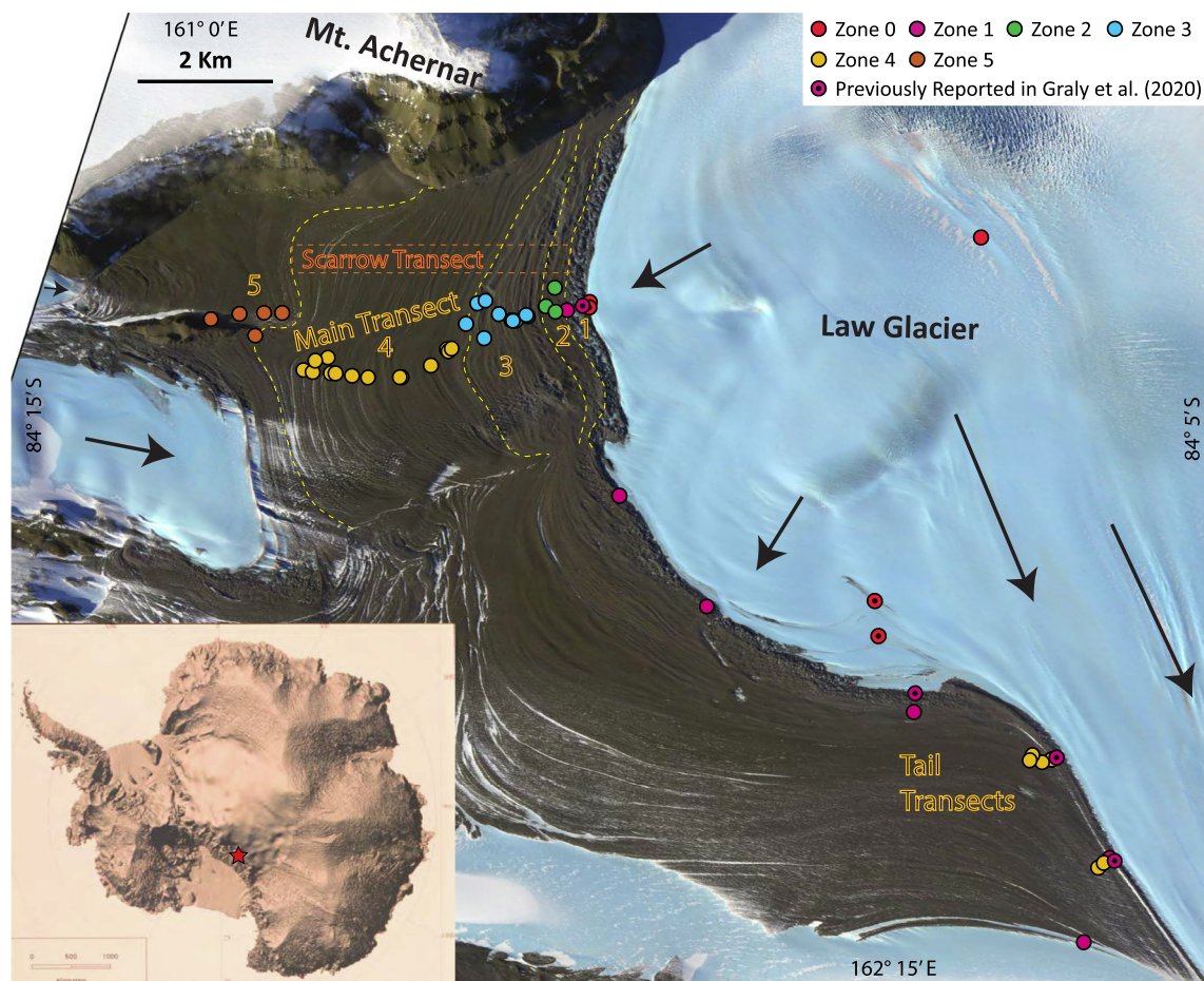
Fig. 1. Sampling locations on Mt. Achnar Moraine, Central Transantarctic Mountains. The main transect is divided into geomorphic zones (numbers labelled) per Bader et al. (2017). The approximate location of the transect collected by Scarrow et al. (2014) is also shown. Approximate down glacier flowlines illustrated with arrows and flow into the moraine. Imagery courtesy of U.S. Polar Geospatial Center.
