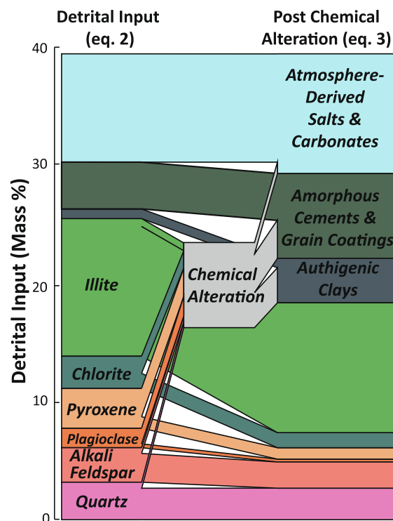
Fig. 10. A solution to the mass inputs as a percentage beyond initial mass and chemical alterations that explains the evolution of mineral and chemical abundance in the <63 \mu\text{m} fraction with time (Figs. 4–6). The left side shows the mineral input in addition to the <63 \mu\text{m} fraction's initial mass that solves for elemental composition after 500 ka of evolution via Eq. (2) (i.e. Fig. 4). Detrital input over the 500 ka period is calculated as 39% above the initial sediment mass. The right side accounts for leaching and alteration on the moraine surface in terms of the 500 ka of mineral abundance evolution via Eq. (3) (i.e. Fig. 5). This solution minimizes the mass input required; other solutions are found in Appendix C.
