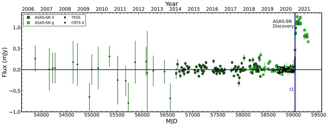
Figure 3. Long-term host-subtracted light curve of NGC 6297 from CRTS, ASAS-SN, and TESS. Dark green circles show CRTS V-band data stacked in 50 days bins. Squares represent ASAS-SN photometry, with dark green showing V-band data and light green showing g-band data. The ASAS-SN data is stacked in 10 days bins prior to the flare and 5 days bins after the flare. Red diamonds show TESS data in 2 hr bins. The horizontal black line represents zero flux. The vertical blue line is the time of first light obtained from our fit to the TESS data, and the vertical black line marks the time of the ASAS-SN discovery.
