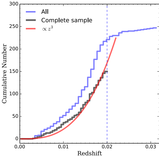
Figure 1. The cumulative redshift distribution of all SNe Ia (blue histogram) in DR1 and those in the complete sample (black histogram) from the CNIa0.02 project. The redshift limit of z = 0.02 for the complete sample is indicated with the dashed vertical blue line. An illustrative N \propto z^3 is plotted with the red line to indicate a simplified expectation from a volume-limited sample covering the full luminosity range by assuming a linear relation between distance and redshift. The distribution approximately follows the expectation for a volume-limited sample at z \gtrsim 0.01 , for which peculiar velocities are negligible compared to the Hubble expansion velocity. The apparent excess of SNe with 0.005 \lesssim z \lesssim 0.013 with respect to the volume-limited expectation is probably contributed by the effects of peculiar velocities at low redshift and/or fluctuations due to small number statistics.
