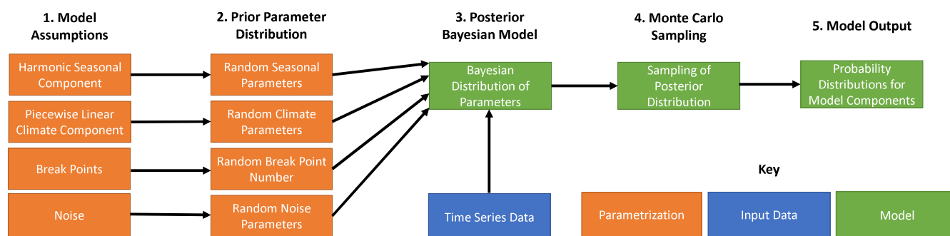
FIGURE 4 A schematic representation of the Rbeast model [Colour figure can be viewed at wileyonlinelibrary.com ]
