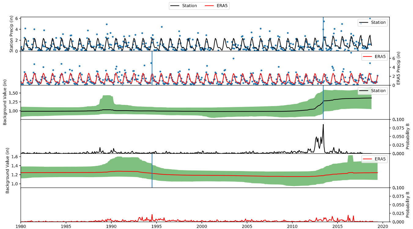
FIGURE 6 A comparison between the university experimental station and ERA5 reanalysis covering the period (1979–2018). The top panel shows the station data and corresponding Rbeast model fit while the second panel displays the same information for the reanalysis data. The middle two panels show the background component and corresponding change point probability distribution for the station data while the bottom two panels show the same data for the reanalysis output. Note that there is some missing data left blank in the station data series in 2003 [Colour figure can be viewed at wileyonlinelibrary.com ]
