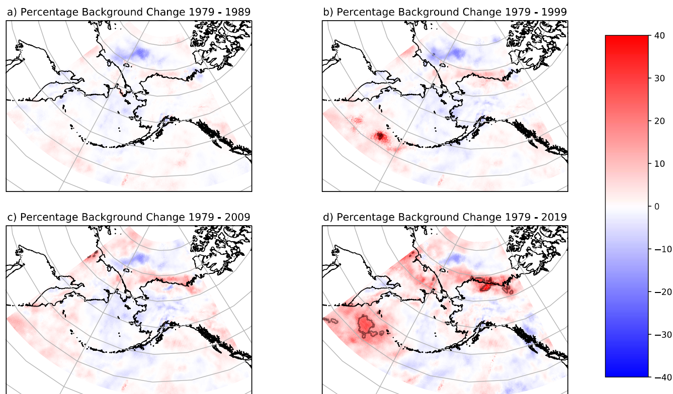
FIGURE 12 Maps showing percentage change in background precipitation over time according to Rbeast. Each panel shows the percentage change in the background component relative to the record start in 1979 and the end year indicated above the panel. Grid cells where the 95% credible interval no longer overlaps (indicating high confidence in change) are outlined in black [Colour figure can be viewed at wileyonlinelibrary.com ]
