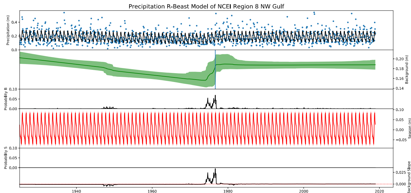
FIGURE 5 An example of Rbeast output for NCEI Region 8 (Northwest Gulf of Alaska) using monthly precipitation totals over the period (1925–2018). The top panel shows the best fit model results alongside the input time series data points. The second panel shows the best fit background component surrounded by a 95% credible interval derived from the sample distribution. Model identified changepoints are marked with vertical blue lines. The third panel shows the probability distribution that any given point represents a changepoint. Note how the peaks align with the vertical blue lines. The next two panels mirror the previous two except they depict the harmonic seasonal component rather than the background climate component. The final panel shows the instantaneous slope of the background component to aid in trend identification [Colour figure can be viewed at wileyonlinelibrary.com ]
