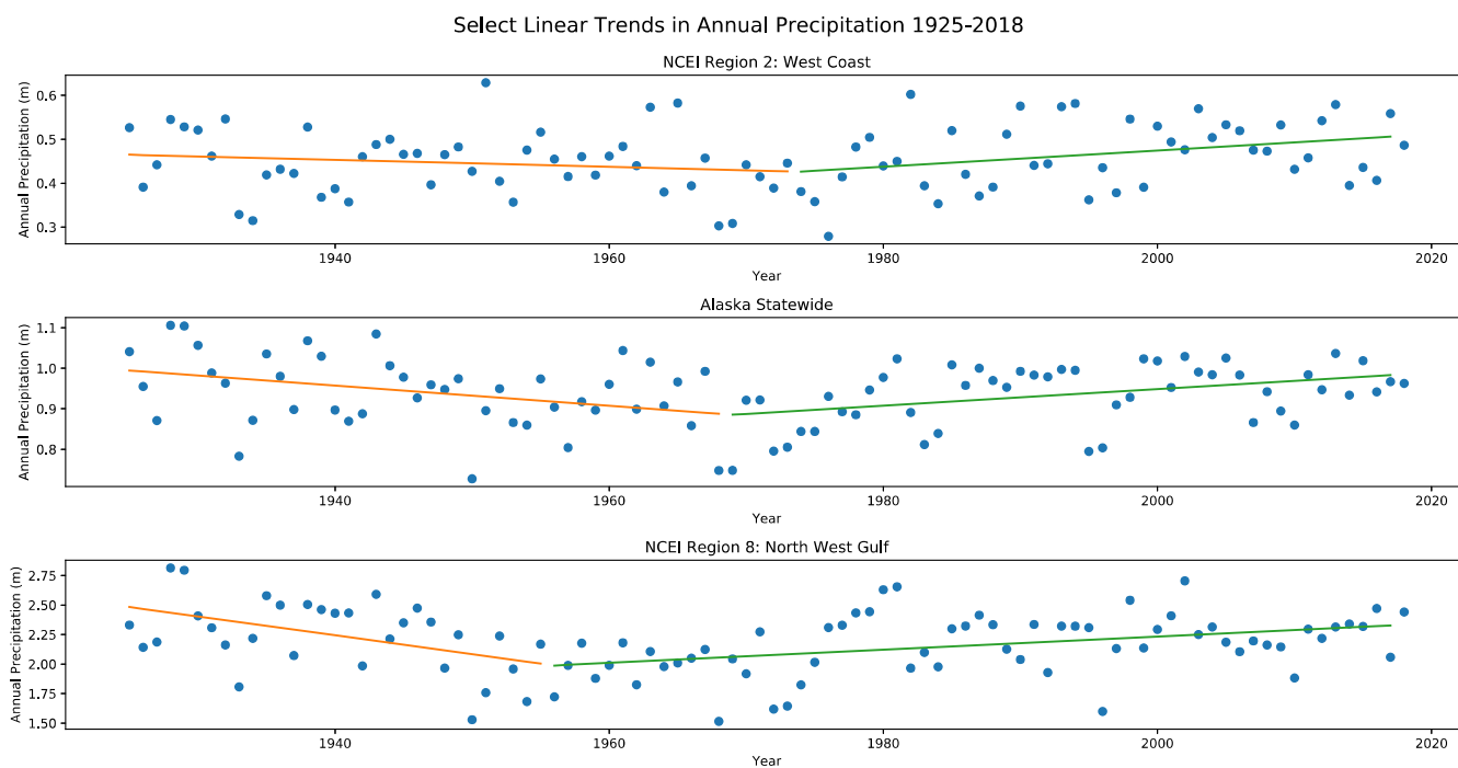
FIGURE 3 As in Figure 2 but for the entire time period (1925–2018) of the NCEI data. A piecewise linear regression model was constructed using methods from Muggeo (2016), which determines the validity of a breakpoint by finding the difference in slopes. The fit is improved by the breakpoint analysis [Colour figure can be viewed at wileyonlinelibrary.com ]
