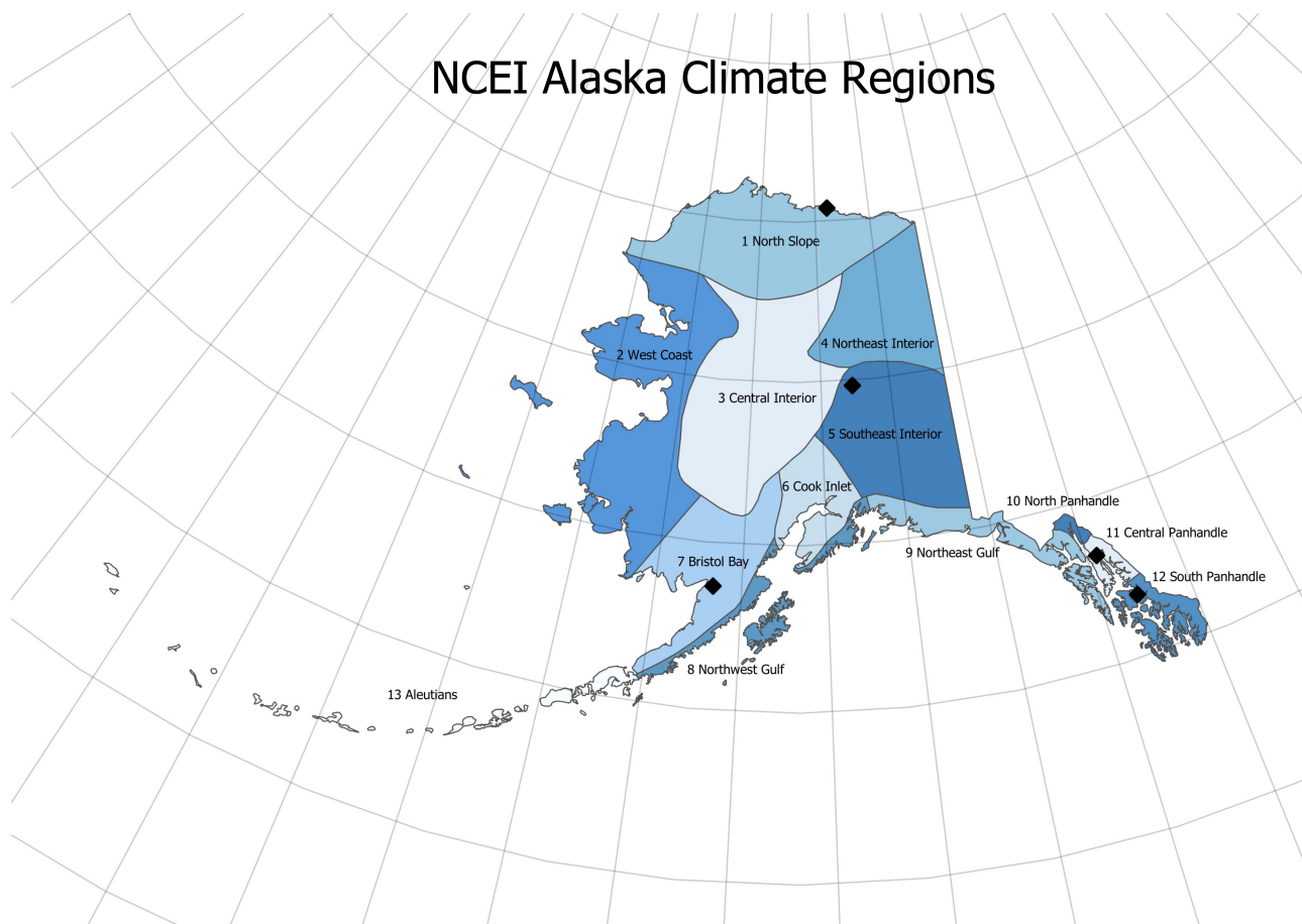
FIGURE 1 A map of the NCEI climate regions. Diamonds indicate stations that are analysed later in this paper. Regions from Bieniek (2012) [Colour figure can be viewed at wileyonlinelibrary.com ]
