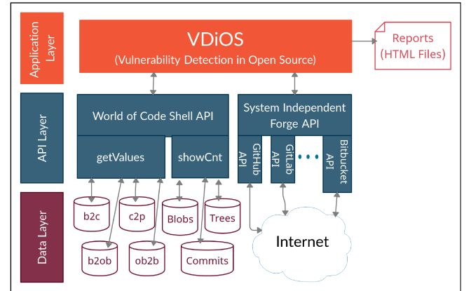
Figure 1: VDiOS Architecture Diagram
