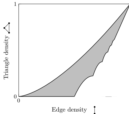
FIGURE 1. The graph profile of edge and triangle
