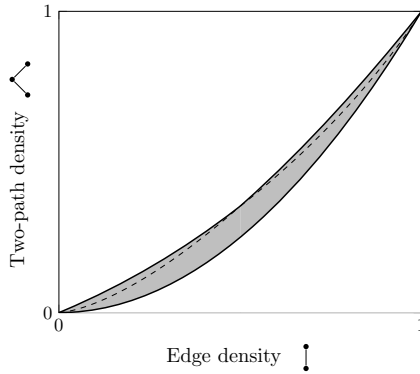
FIGURE 6. The graph profile of \mathcal{V}_1
