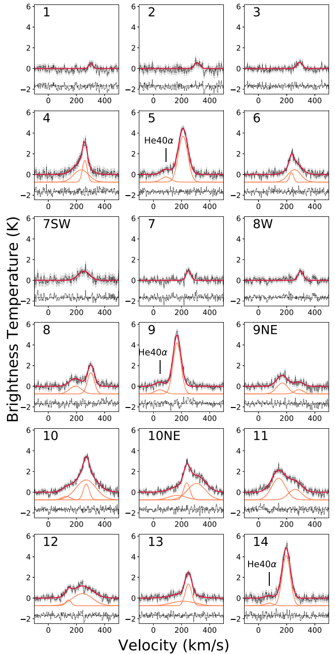
Figure 3. Spectra of H40 \alpha toward all sources labeled in Figure 1. One-, two-, and three-component Gaussian fits are conducted to account for gas at different line-of-sight velocities, and the resulting fit for each spectrum is plotted in red. For sources where there are multiple components fit, the individual Gaussian components are also plotted in orange. Residuals from the fitting are plotted below the spectra. The results of these fits are given in Table 1. The location of the He40 \alpha line is indicated in the three sources (5, 9, and 14) where it is clearly detected.
