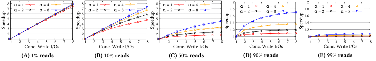
Figure 7: Speedup of an Unbatchable Reads, Batchable Writes application. The speedup is highest for write-intensive workloads. Furthermore, the speedup depends on the device asymmetry – the higher the asymmetry, the higher the speedup.
