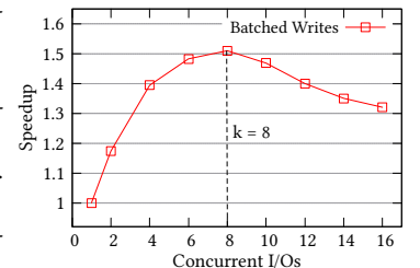
Figure 10: Speedup increases as more concurrent I/Os are used until the device is saturated.
