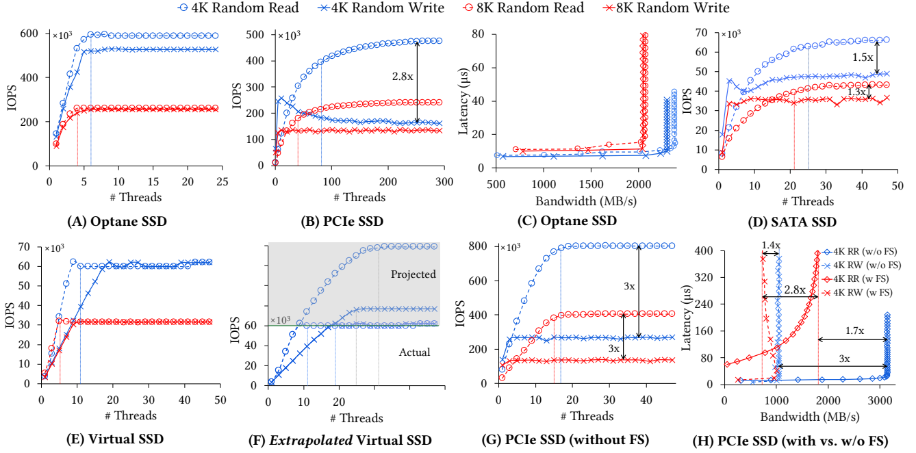
Figure 4: All devices show different degree of k and \alpha depending on the file system, access type, and block size. The benefit of exploiting k can be as high as 40 \times . (A) The Optane SSD has lower k and \alpha \approx 1 . (B) The PCIe SSD shows high k with \alpha up to 2.8. (C) Latency does not increase until saturation. (D) The SATA SSD shows lower k than the PCIe SSD with \alpha up to 1.5. (E) The Virtual SSD is software-controlled, exhibiting \alpha \approx 2 prior to saturation. (F) The extrapolated performance profile of the Virtual SSD following the trends of other SSDs. (G, H) Bypassing the file system allows for 1.7 \times (1.4 \times ) higher read (write) throughput for PCIe SSD, while the values of both \alpha and k are more stable across the experiments.
