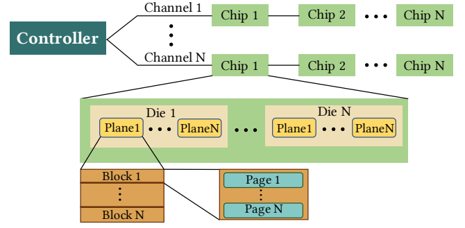
Figure 3: Internal architecture of an SSD.
