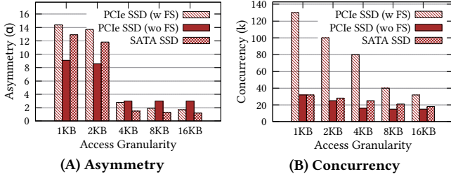
Figure 5: (A) The asymmetry is high when I/O size is smaller than native page size; as I/O size increases \alpha decreases. (B) The concurrency decreases for larger I/O size.
