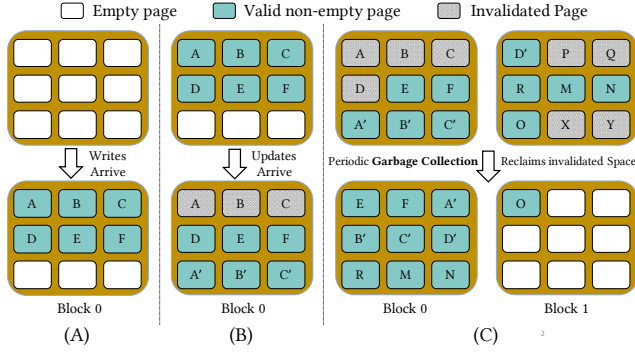
Figure 2: (A) Not all writes are costly; six pages (A-F) are written in a block. (B) Updates cause invalidation of pages which cannot be overwritten unless the whole block is erased. (C) Periodic garbage collection reclaims the invalidated pages.
