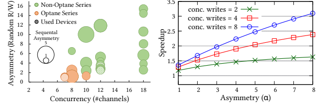
Figure 1: (A) Asymmetry ( \alpha ) and Concurrency ( k ) in recent SSDs; most devices show high \alpha and k . (B) Gain increases as more concurrent I/Os are used, and \alpha dictates the gain.
