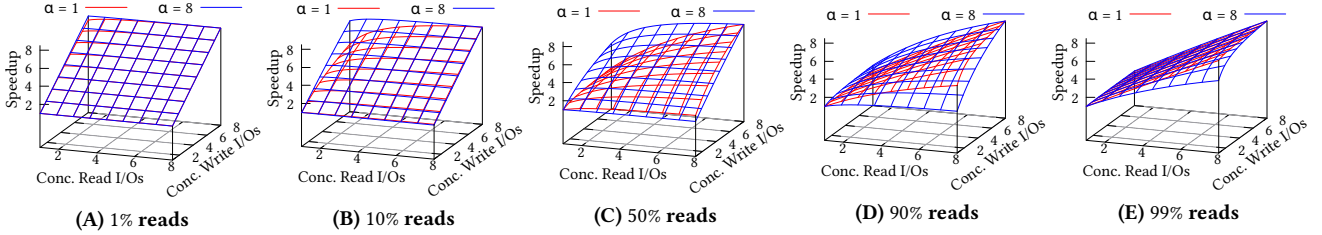
Figure 9: Speedup of a Batchable Reads and Writes application. (A, B) For fewer reads, speedup increases with more conc. write I/Os irrespective of conc. read I/Os. (C, D, E) Read concurrency comes into action as more reads are introduced in the workload.
