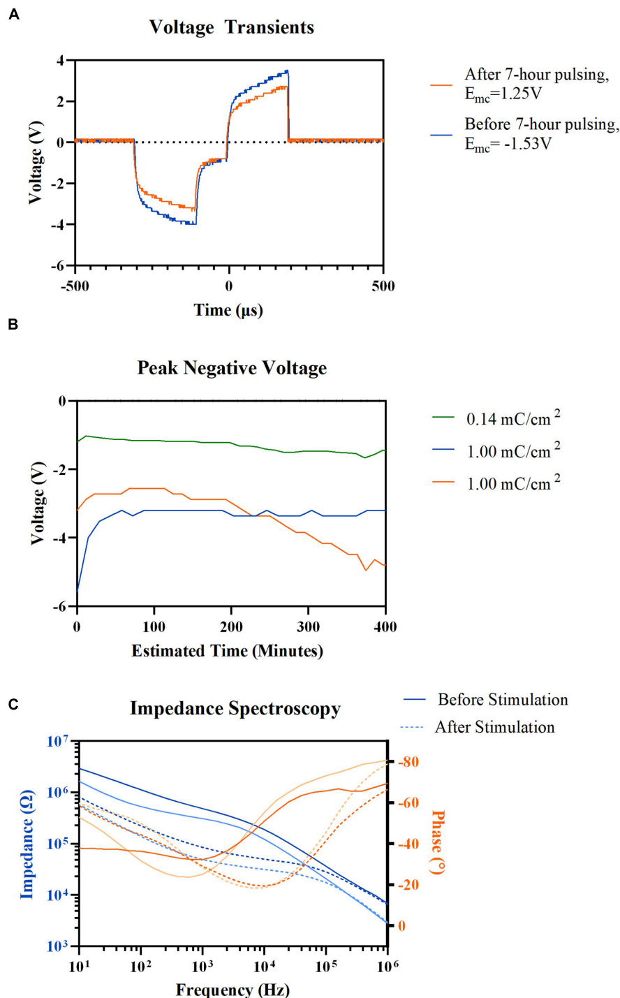
FIGURE 4 | Electrochemical properties recording result before, after, and during 7-h electric stimulation. (A) Representative voltage transient of HDCF electrode before and after 7-h electric stimulation, 1.00 mC/cm^2 current density, 72 \mu A . (B) Voltage transient peak negative values measured during cathodic phase of electric stimulation in three different HDCF electrodes: (green) 0.14 mC/cm^2 , (blue) 1.00 mC/cm^2 , and (orange) 1.00 mC/cm^2 . (C) Pre-(Solid lines) and post-stimulation (Dotted lines) electrochemical impedance spectroscopy results of two HDCF electrodes (Blue) Impedance values and (Orange) Electrode frequency values.
