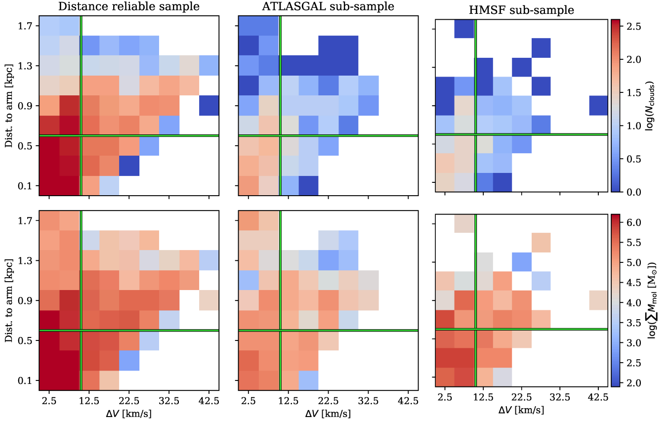
Fig. 7. Bi-dimensional histograms of the total number of cloud counts ( top row ) and cumulative molecular gas mass in clouds ( bottom row ) within bins of 0.1 kpc and 0.25 km s -1 , considering the xy -plane distance and the velocity offset to the closest spiral arm. Different cloud subsamples are considered: the distance-reliable sample ( left ), the subset of this sample that contains an ATLASGAL source ( middle ), and the subset with a high-mass-star-formation (HMSF) signpost ( right ). The vertical green line indicates the \Delta V = 10 km s -1 that we use to define a spiral arm, and the horizontal green line indicates the median spiral width of 580 pc.
