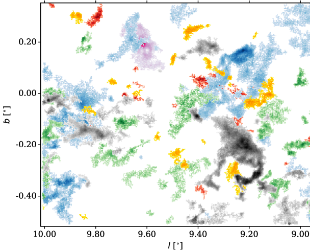
Fig. 3. Multi-coloured integrated intensity maps of the ^{13}\text{CO} (2–1) emission in an inset of the ‘G009’ SEDIGISM field. Clouds attributed to a given spiral arm are colour-coded: magenta (3 kpc), red (Norma-Outer), blue (Scutum-Centaurus), green (Sagittarius-Carina), yellow (Perseus), grey (inter-arm or unreliable distance clouds). For visualisation purposes, in these images, we include also clouds attributed to the 3 kpc arms and with uncertain location, even if they are not used in further analyses. The same images for the full survey are collected in Appendix E.
