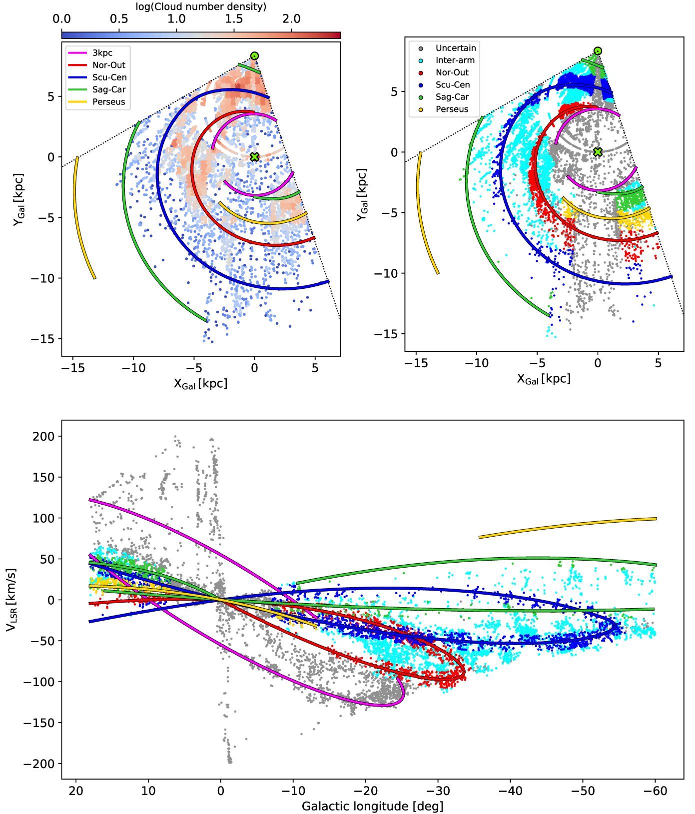
Fig. 2. Face-on view of the Galactic region surveyed by SEDIGISM (confined within the dotted lines; top panels ) overlaid with spiral arm tracks defined by TC93: the 3 kpc arms in magenta, the Norma-Outer arm in red, the Scutum-Centaurus arm in blue, the Sagittarius-Carina arm in green, and the Perseus arm in yellow (the solid lines merely trace the bottom of the potential, and do not correspond to a real ‘thickness’). The position of the Sun is indicated with a green circle, while the Galactic centre is shown with a green ‘X’. In the top-left panel, coloured dots represent the number density distribution of all molecular clouds identified within the SEDIGISM field by DC21. The top-right and bottom panels show the distribution of the clouds in the full sample with respect to the spiral arms in xy and lv space, respectively. Clouds are colour-encoded by the attributed spiral arm. Objects in the inter-arm region are in cyan and clouds with uncertain allocation are shown in grey. The latter consist of clouds associated with the 3 kpc arms and those with unreliable distances.
