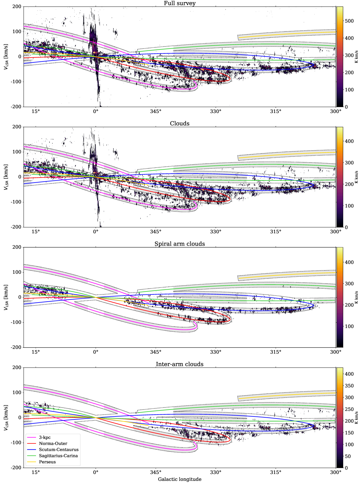
Fig. 1. From top to bottom: longitude–velocity map ( lv -map) from the trunk-masked full survey data cube (see Sect. 2), the cloud data cube, the data cube obtained for the clouds located in the spiral arms, and the data cube obtained for the clouds located in the inter-arms (following the C_{xy}A method described in Sect. 4.2.2). In each panel, the spiral arm tracks defined by Taylor & Cordes (1993) are overlaid: the 3 kpc arms in magenta, the Norma-Outer arm in red, the Scutum-Centaurus arm in blue, the Sagittarius-Carina arm in green, and the Perseus arm in yellow. Dotted black lines surround areas of the lv -map that have a velocity offset with respect to the spiral arms within 10 \text{ km s}^{-1} . Shaded patches indicate regions along the spiral arms where the velocity difference between adjacent arms (along the velocity axis) is greater than 20 \text{ km s}^{-1} . In the last two panels, the clouds associated with the 3 kpc arms and the clouds with unreliable distance are excluded as they cannot be unequivocally associated with a spiral arm or inter-arm region (see Sect. 4.2.2).
