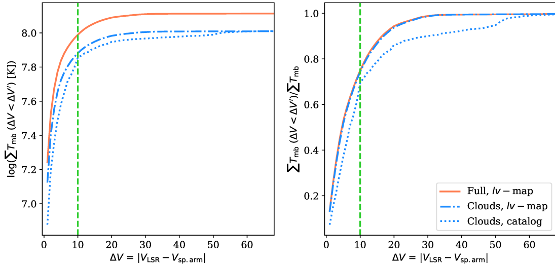
Fig. 5. Cumulative distribution of the integrated intensity of the velocity offsets with respect to spiral arms ( \Delta V ; left ) and cumulative distribution normalised by the total flux in their respective datasets ( right ). In the panels, we show cumulative distribution from the different methods described in the text: direct integration of the original lv -map data cube (orange full line), integration of the lv -map generated by cloud masks (blue dotted-dashed line), integration of the cloud fluxes as per their cloud velocity centroid association to the closest spiral arm (blue dotted lines). The dashed green line shows the 10 \text{ km s}^{-1} width used to define arm association.
