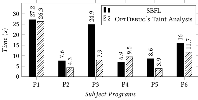
Figure 9: OPTDEBUG’s taint analysis on a simplified input is on average 27% faster than applying spectra-based fault localization on a simplified input.
