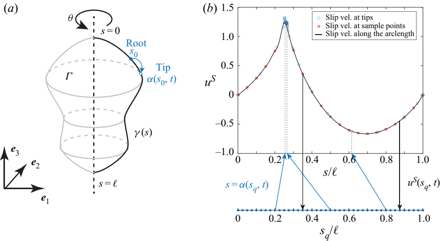
Figure 1. (a) Schematic of the microswimmer geometry. The shape is assumed to be axisymmetric, obtained by rotating the generating curve \gamma about the \mathbf{e}_3 axis. The tip of the cilium rooted at s_0 at time t is given by s = \alpha(s_0, t) . (b) Illustration of the algorithm for computing the slip velocity at the quadrature points u^S(s_q, t) . We first compute the ‘tip’ position and the corresponding tip velocities (open blue circles) of cilia rooted at the N_q quadrature points s_q (closed blue circles). We then obtain the slip velocities at sample points uniformly distributed along the generating curve (open red squares) by a cubic interpolation. The slip velocity at any arc length (black curve) is then obtained by a high-order B-spline interpolation from the sample points. We have reduced the number of quadrature and sample points in this figure (compared to values used in the numerical experiments) to avoid visual clutter.
