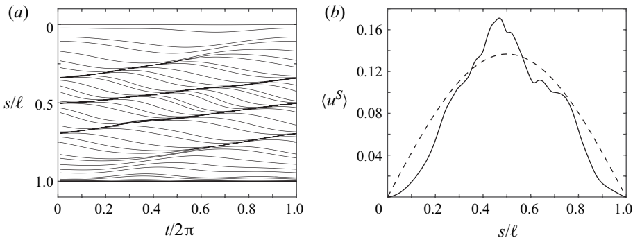
Figure 4. Ciliary motion (a) and mean slip velocity (b) for the optimal spherical swimmer with constraint ( \Delta s_{max}/l \approx 5.0\% ). The efficiency is \epsilon \approx 6.9\% and the swim speed is \langle U \rangle \approx 0.091 . The swimmer forms multiple waves in the equatorial region, leading to a high slip velocity at s \approx 0.5l . The motion close to the poles is nearly zero. The dashed curve in (b) is the time-independent optimal slip velocity of the spherical swimmer, scaled by the swim speed. The video of the optimal ciliary motion can be found in the online supplementary material (Movie 3).
