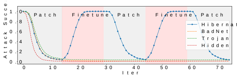
Figure 5: Comparison of ASR during recursively patching and fine-tuning.
