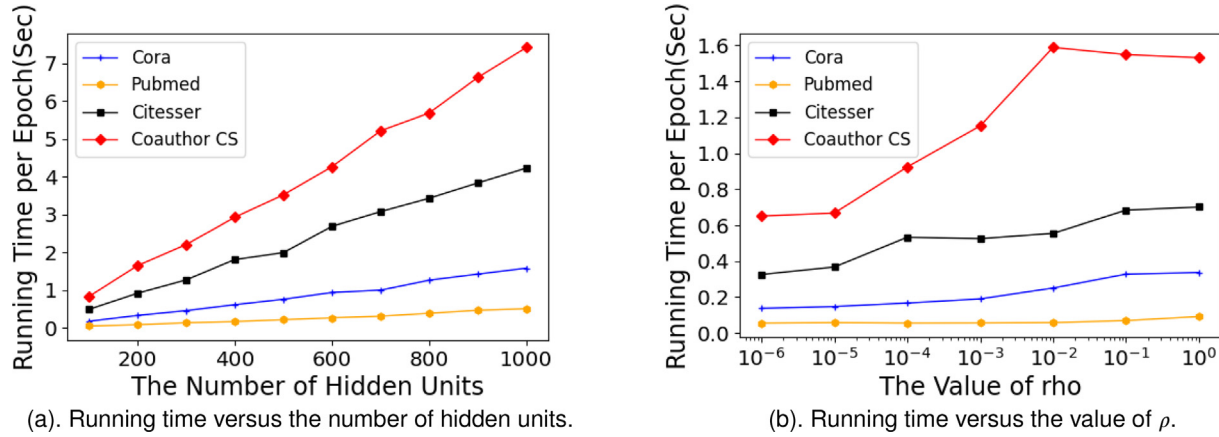
Fig. 3. The relationship between the running time and: (a) the number of hidden units; (b) the value of \rho : the running time increases linearly with them in general.
