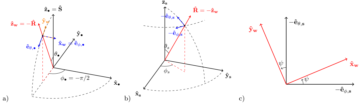
FIG. 1. Conventions for the source frame, solar system baricenter frame, and polarization angle are shown in the schematic diagram above. For the source-frame diagram (a), the coordinate basis is defined in Eq. (7). The direction towards the solar system baricenter ( -\hat{\mathbf{R}} ) is shown as the red arrow which defines \hat{\mathbf{z}}_w . The source-frame polarization vectors are shown in blue and the basis vectors in the wave frame (see Eq. 6) are shown in orange. Note the rotation by \pi/2 to align the source-frame polarization vectors with the wave-frame basis. Also, due to conventions chosen, \phi_\bullet = -\pi/2 always. In the solar system baricenter frame (b), the solar system baricenter frame polarization basis is shown in blue. The red arrow shows the angle to the source ( +\hat{\mathbf{R}} ). Finally, in plot (c), the polarization determination is illustrated. The polarization angle represents the rotation down the line-of-sight from the wave-frame (red) to the solar system baricenter polarization basis (black).
