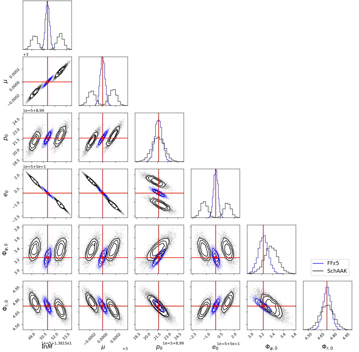
FIG. 10. Corner plot showing one- and two-dimensional marginalized posteriors for an injection with (M, \mu, p_0, e_0, \Phi_{\phi,0}, \Phi_{r,0}) = (10^6 M_\odot, 3M_\odot, 8.99, 0.5, 3.23, 4.72) . The histograms and contours for the \epsilon = 10^{-5} fast FEW (FF \epsilon 5) and Schwarzschild AAK (SchAAK) template waveforms are shown in blue and black, respectively. The true injection parameters are denoted with the red vertical and horizontal lines. Note the sampling methods used concentrated near the true value. The samplers are not be able to access secondary modes with a strong separation from the injection point. Due to the inaccuracy of the semi-relativistic amplitudes in the SchAAK waveform, a strong bias and multimodal behavior are observed when fitting a SchAAK waveform template against an FF \epsilon 5 relativistic injection. The consequences of this behavior are further discussed in Section VII.
