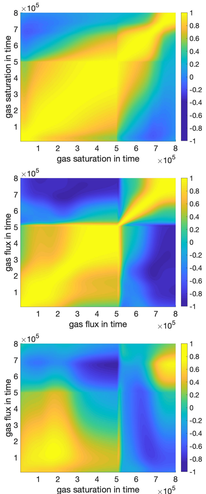
Fig. 19 Top: correlation matrix for S_{N_{qoi}}^{PC}(t, \xi^r) computed using the analytic formula in Eq. 27, middle: correlation matrix for Q_{N_{qoi}}^{PC}(t, \xi^r) computed using the analytic formula in Eq. 27, bottom: cross-correlation structure of S_{N_{qoi}}^{PC}(t, \xi^r) and Q_{N_{qoi}}^{PC}(t, \xi^r) computed using the analytic formula in Eq. 28
