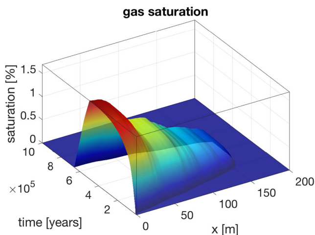
Fig. 7 Space time evolution of gas saturation
