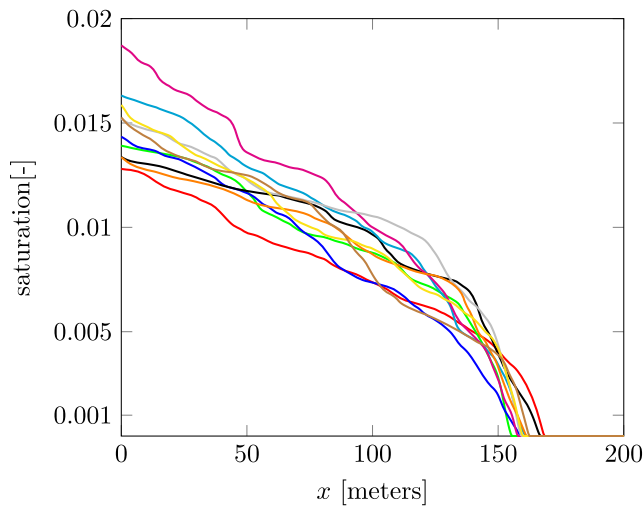
Fig. 6 Gas saturation at t^* = 300,091 years
