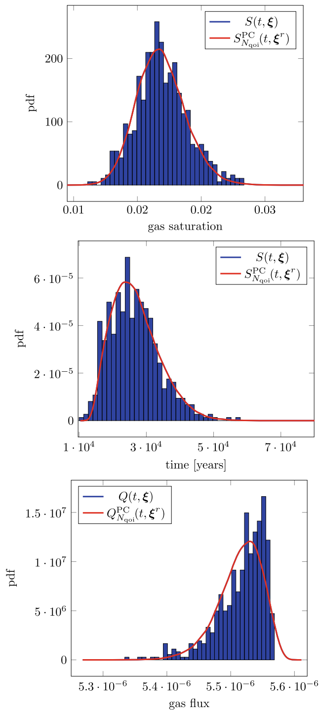
Fig. 18 Comparison of normalized histograms and pdf estimates for top: max saturation value of S_{\max} , middle: first time S_{N_{qoi}}^{PC}(t, \xi^r) is above 20% S_{\max} , bottom: max flux value Q_{\max}
