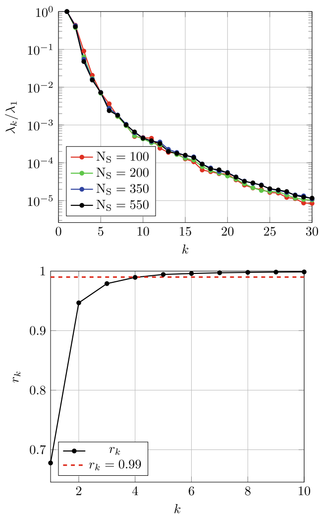
Fig. 10 Top: comparison of ratio \lambda_k/\lambda_1 , k = 1, \dots, 30 for \lambda_i(C_{\text{qoi}}) corresponding to S(t, \xi) computed with various sample sizes, bottom: r_k as defined in Eq. 13, k = 1, \dots, 10 , for S(t, \xi) . Dotted line corresponds to 0.99
