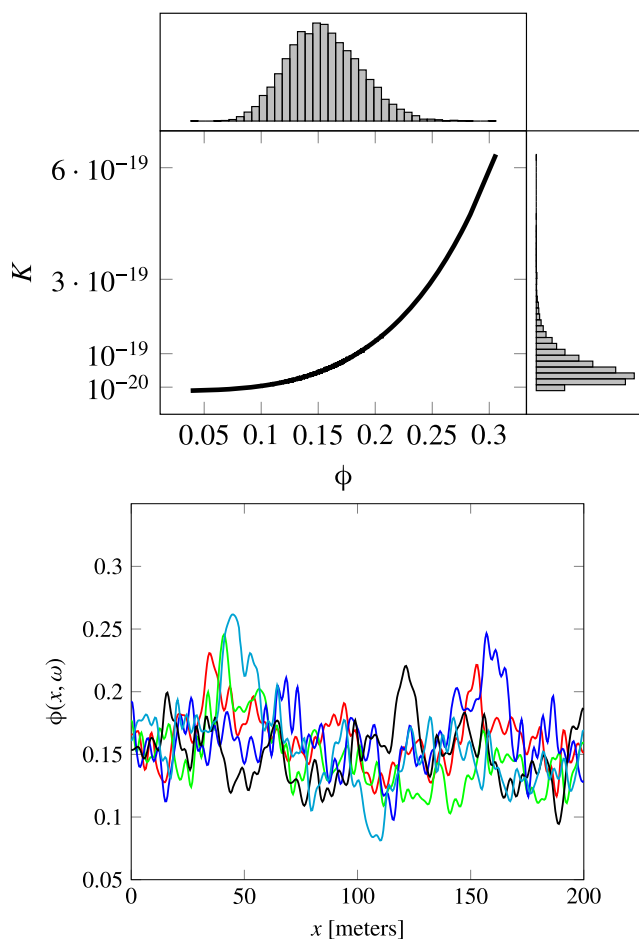
Fig. 4 Top: the porosity permeability relation and the distributions of pointwise porosity and permeability. Bottom: a few realizations of the porosity field
