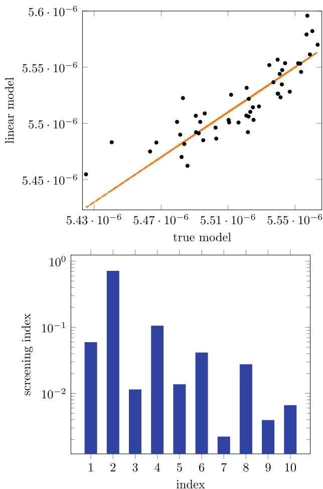
Fig. 13 Top: comparison of the true model to the linear model for Q(t, \xi) at t = 500,106 years, bottom: screening indices for Q(t, \xi)
