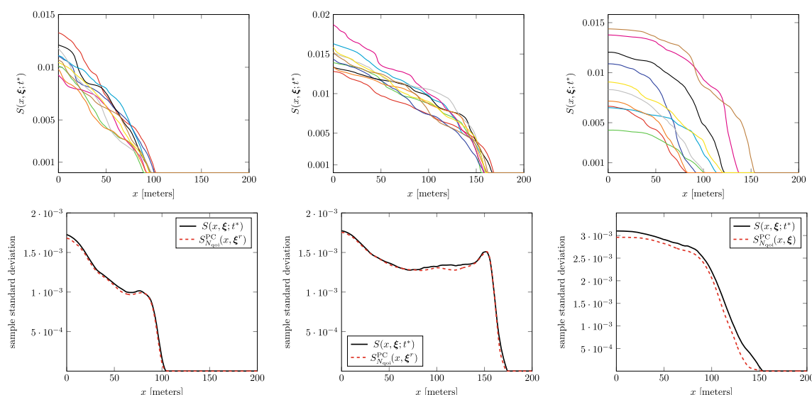
Fig. 17 Top row, left to right: sample realizations of S(x, \xi; t^*) for times 100,099, 300,091, and 600,043 years; bottom row, left to right: comparison of sample standard deviation of S(x, \xi; t^*) and S_{N_{qoi}}^{PC}(x, \xi; t^*) computed on 200 sample points
