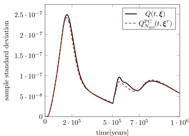
Fig. 15 Comparison of sample standard deviations of Q(t, \xi) and Q_{N_{qoi}}^{PC}(t, \xi^r) computed with 200 sample points
