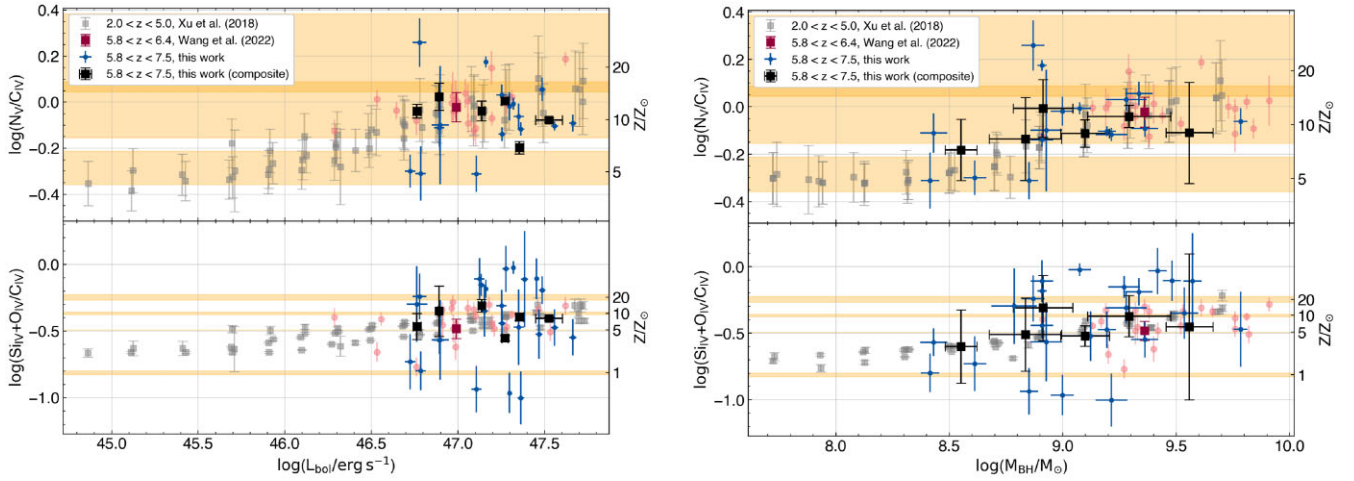
Figure 6. N\text{ IV}/C\text{ IV} and (\text{Si IV} + \text{O IV})/C\text{ IV} flux ratios as a function of the quasar bolometric luminosity (left-hand panel) and virially estimated black hole mass (right-hand panel). The low-redshift sample ( 2.0 < z < 5.0 ) indicated in grey is from Xu et al. (2018) while another higher redshift comparison sample indicated in red is sourced from Wang et al. (2022). Our sample is presented in blue and black. Square points with capped error bars indicate composites while circular points indicate individual fits. Not all individual quasars involved in the composites are plotted. The single red square denotes the composite from Wang et al. (2022). The black hole masses in this study and in Wang et al. (2022) are estimated with single-epoch virial estimates using the \text{Mg II} emission line, while the Xu et al. (2018) study uses the C\text{ IV} emission line. The orange shaded space indicates a range of line ratios which are consistent with the metallicity indicated in the secondary axis based on photoionization calculations with different ionizing SEDs. The overlapping region in the N\text{ IV}/C\text{ IV} plot indicates a range of line ratios which is consistent with both Z = 10 and 20 Z_\odot (e.g. Hamann et al. 2002; Nagao et al. 2006). Metallicity values larger than 10 Z_\odot are extrapolated.
