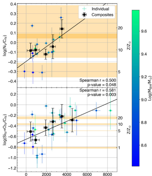
Figure 8. N\text{ V}/C\text{ IV} and (\text{Si IV} + \text{O IV})/C\text{ IV} flux ratios as a function of the C IV blueshift of quasars in the sample. Blueshift composites are presented in black while individual fits are mapped on to a blue–green gradient scaled to the black hole mass. The minimum C IV blueshift error is 200\text{ km s}^{-1} based on the 1\text{ \AA} wavelength bins, but the contribution from the systemic redshift error is added in quadrature for an average total of 230\text{ km s}^{-1} uncertainty. The Spearman correlation coefficients and p -values are derived from the fits to individual quasars. The orange shaded space indicates a range of line ratios which are consistent with the metallicity indicated in the secondary axis based on photoionization calculations with different ionizing SEDs. The overlapping region in the N\text{ V}/C\text{ IV} plot indicates a sub-space of parameters which is consistent with both Z = 10 and 20Z_{\odot} . The line ratio correlation with the C IV blueshift is more significant than the correlation with black hole mass or bolometric luminosity.
