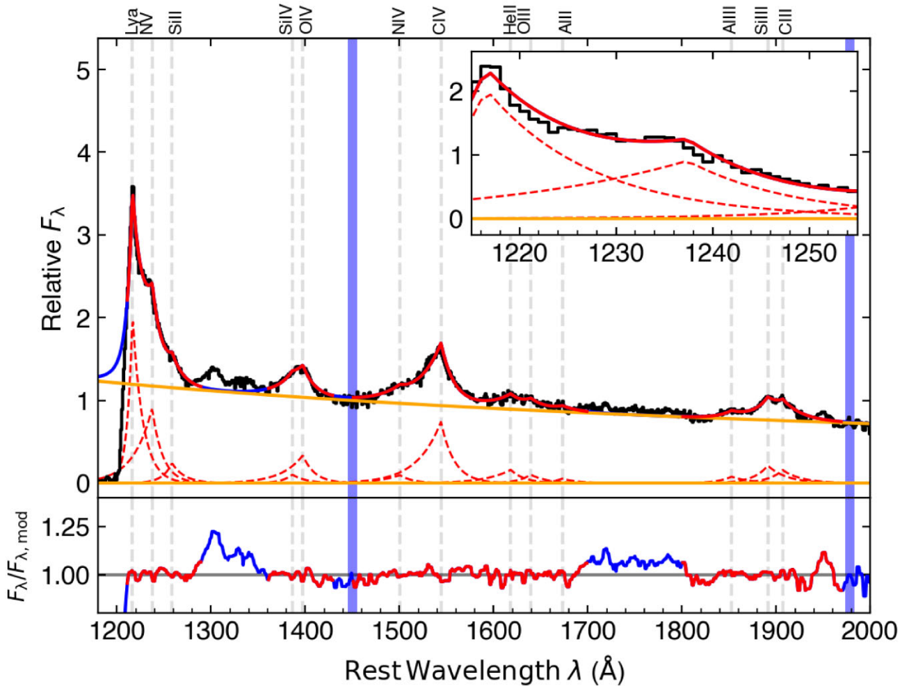
Figure 4. Example fit to ATLASJ029-36 observed using VLT/X-shooter with a mean SNR per 1 Å pixel of 27.35 between 1400–1600 Å. The top plot shows the spectrum after the post-processing techniques and the bottom plot shows the residuals. The inset plot provides a closer look at the line profiles of Ly \alpha and N V. The vertical blue bars indicate the continuum fitting windows, which are fit by the power-law continuum denoted by the orange line. The red lines indicate the emission line fits as well as the extent of the individual line-fitting windows. All fitted emission lines are labelled and their individual line profiles are shown.
