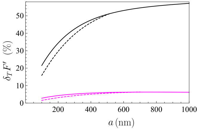
FIG. 6. The computational results for the relative thermal correction to the gradient of the Casimir force are shown as functions of separation by the bottom and top pairs of lines for an Au-coated sphere interacting either with real graphene sheet deposited on a SiO 2 plate or with freestanding real graphene sheet in vacuum, respectively. The solid and dashed lines in each pair are computed including and neglecting the explicit dependence of the polarization tensor on temperature as a parameter, respectively.
