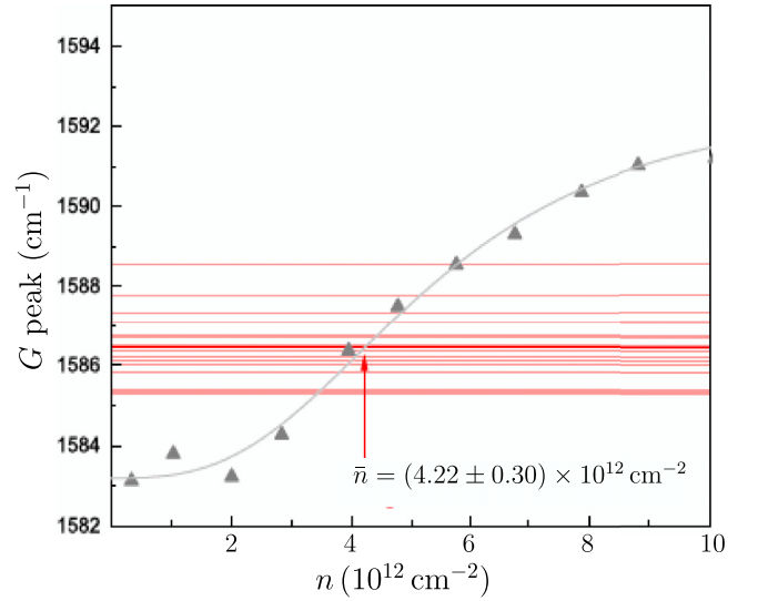
FIG. 3. The measured G -peak values from Raman spectroscopy compared to the charge concentration in graphene from Ref. [91]. The solid triangles are the values from Ref. [91] and the solid gray line is a best fit to the data. The G -peak values measured at equidistant points on the sample are shown by horizontal lines. The intersection identifies the impurity concentration. The average impurity concentration is shown by the arrow.
