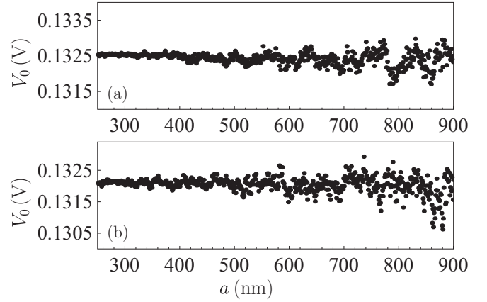
FIG. 1. The residual potential difference between an Au-coated sphere and a graphene-coated fused silica plate is shown by the dots as a function of separation (a) for the first and (b) second measurement sets.
