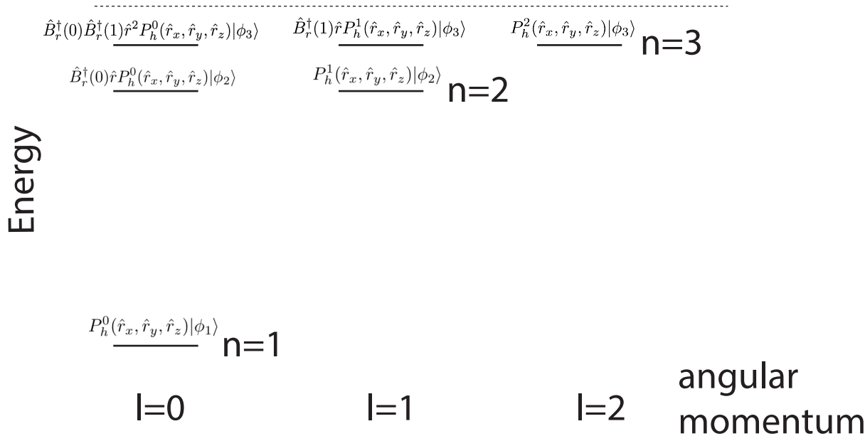
Figure 1. First three energy eigenstate multiplets, plotted to show the energy and the corresponding state, along with the angular momentum. The energies are the same for all inequivalent harmonic polynomials with the same l value. The dotted line is the limit point for the energy eigenvalues.
