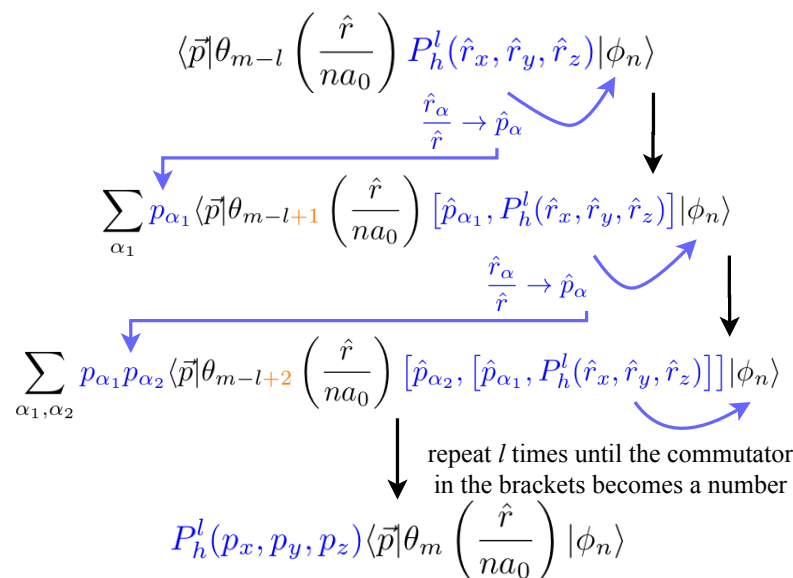
Figure 3. Schematic for how to remove the harmonic polynomial from the operator matrix element to determine the wavefunction in momentum space. Here, \theta is a reverse Bessel polynomial and P_h^l is a harmonic polynomial.
