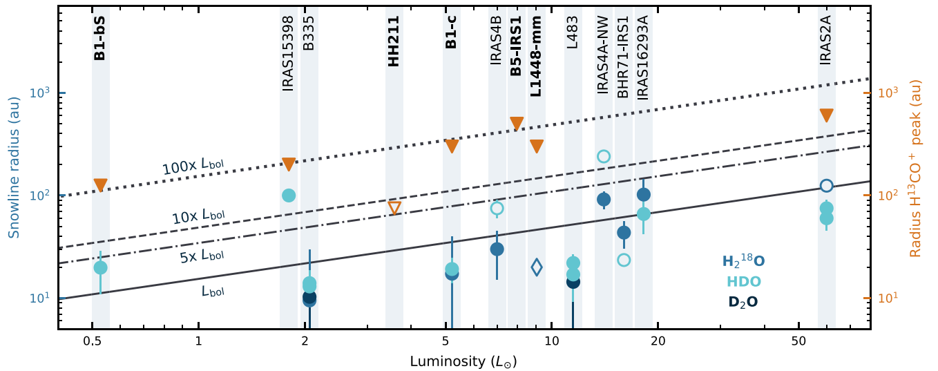
Figure 7. Overview of the constraints on the water snowline location in the protostellar envelopes based on \text{H}^{13}\text{CO}^+ and/or water ( \text{H}_2^{18}\text{O} , HDO, or \text{D}_2\text{O} ) observations. The peak of the \text{H}^{13}\text{CO}^+ emission ( J = 4-3 for IRAS 15398, J = 3-2 for B1-bS, and NGC 1333-IRAS 2A, and J = 2-1 for the other sources), which serves as an upper limit of the snowline location, is shown as orange triangles. The tentative peak for HH 211 is indicated by an open triangle. The snowline location derived from water observations is marked with a circle (blue for \text{H}_2^{18}\text{O} , light blue for HDO, and dark blue for \text{D}_2\text{O} ). Open circles indicate the presence of an outflow contribution. The snowline location derived for L1448-mm based on similarities in emission morphology to B1-c is marked with an open blue diamond. The expected snowline location based on bolometric luminosity (Equation (3)) is indicated by the solid line. The dashed-dotted, dashed, and dotted lines indicate the expected snowline locations if the source has recently undergone an accretion burst that increased the luminosity by a factor of 5, 10, or 100, respectively. A source is considered to have recently undergone a burst if the snowline corresponds to a luminosity > 5 \times L_{\text{current}} . Names of sources studied in this work are highlighted in boldface, and Table G1 lists references for sources not studied here.
