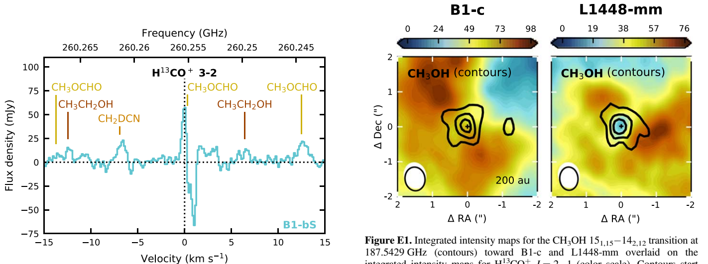
Figure D3. Spectra extracted within a circular 0''.5 diameter aperture ( \sim one beam) toward the continuum peak position of B1-bS centered around the \text{H}^{13}\text{CO}^+ J=3-2 transition.
