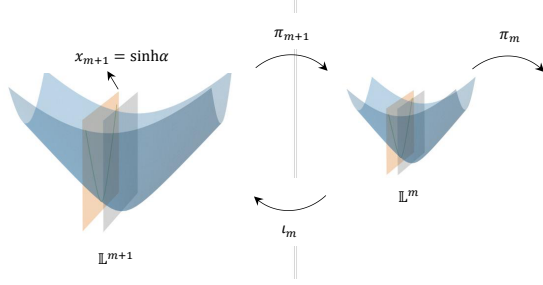
Figure 3. Illustration of NH model using the embedding \iota_m in Eq. (9) of \mathbb{L}^m into \mathbb{L}^{m+1} . The m -dimensional nested hyperboloid in \mathbb{L}^{m+1} is indeed the intersection of \mathbb{L}^{m+1} and an m -dimensional hyperplane.
