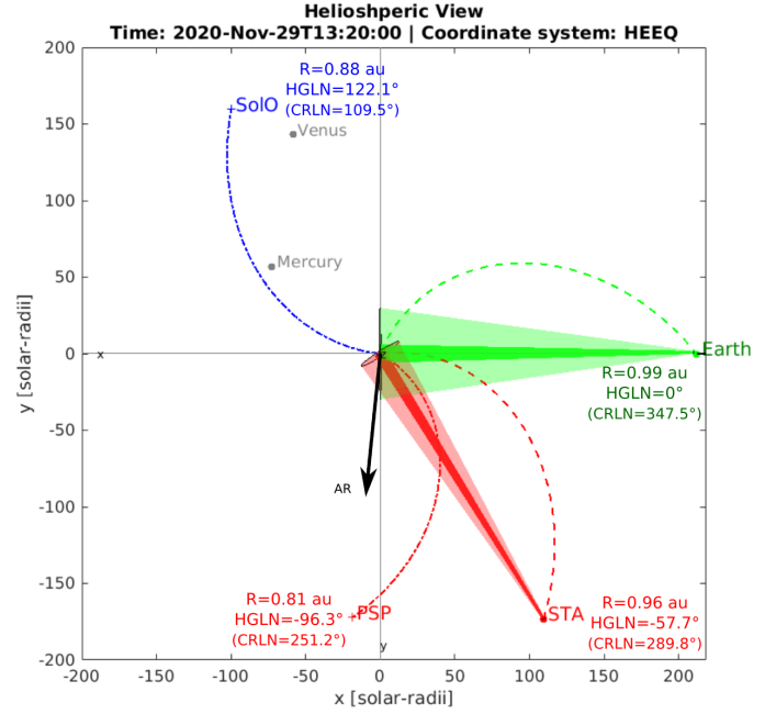
Fig. 1. View of the ecliptic plane from solar north showing the locations of the Sun, Earth, PSP, SoLo, and STEREO-A in the HEEQ coordinate system on 2020 November 29 at 13:20 UT. The fields of view of STEREO-A/COR1 and COR2 and SOHO/LASCO-C2 and C3 are depicted as shaded areas in red and green, respectively. Positions are given by the labels next to each spacecraft or planet marker. The location of the parent AR12790 is indicated by the black arrow. The Parker spirals for the solar wind speed measured by each spacecraft at the time of the eruption are shown by the lines connecting the spacecraft to the solar surface.
