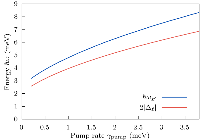
FIG. 7. Comparison of the absorptivity minimum \hbar\omega_B and the BCS-like gap 2\Delta_\ell as a function of the pump rate \gamma_{\text{pump}} for the data shown in Fig. 6. The light red line denotes the magnitude of the BCS-like gap 2\Delta_\ell . The dark blue line shows the frequency \hbar\omega_B for which the real part of the conductivity \text{Re } \sigma_{Tv}(\omega) is a minimum; that is, \hbar\omega_B is defined such that \text{Re } \sigma_{Tv}(\omega_B) = \min \text{Re } \sigma_{Tv}(\omega) . The plot shows that the BCS-like gap is closely tracked by the gain maximum, over a wide range of pumping rates.
