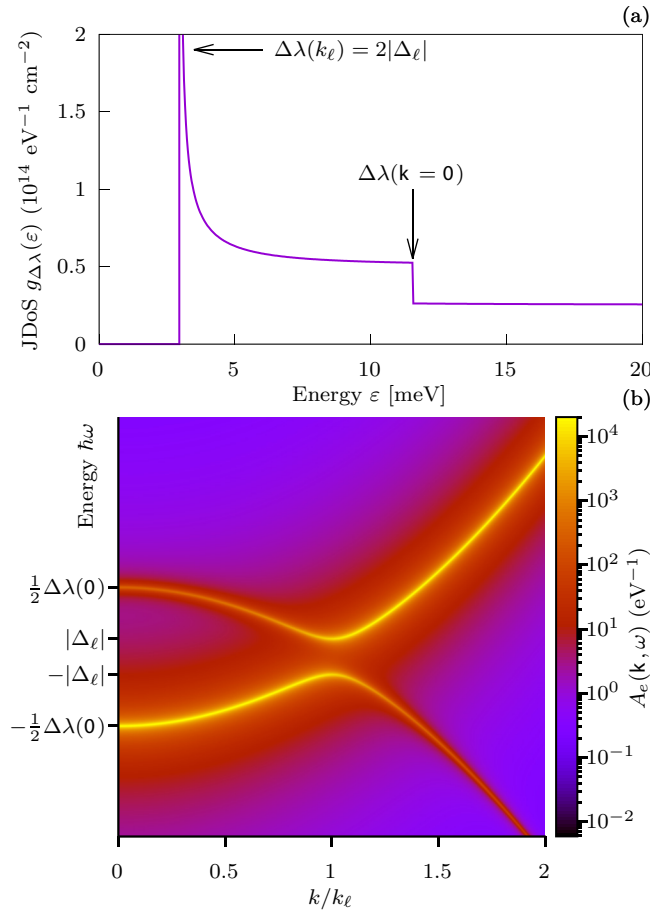
FIG. 4. (a) Joint density of states for transitions between the lower and upper branches of the renormalized conduction band. (b) Color map of the spectral function from Eq. (36) [cf. Eq. (30) of Ref. [49]]. For this and all subsequent figures, the parameters are given in Table I, unless noted otherwise.
