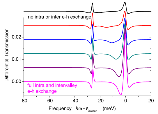
FIG. 10. Differential transmission in the cross-circular configuration ranging from zero intravalley and intervalley exchange to full intravalley and intervalley exchange, \eta_{\text{inter}} = \eta_{\text{intra}} = 0, 0.2, 0.4, 0.6, 0.8 , and 1 from top to bottom. Except for the bottom curve ( \eta = 1 ), the spectra are shifted vertically for clarity. In contrast to the previous DT figures, here the trion is taken into account. The DT response of the trion can clearly be seen at approximately 26 meV below the exciton. Effects of e -h exchange in the trion are omitted.
