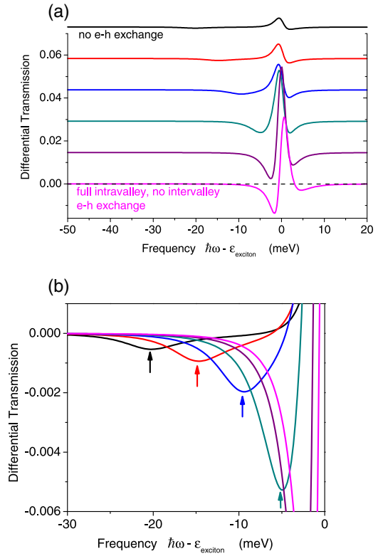
FIG. 2. (a) Differential transmission in the cross-circular configuration without intervalley e -h exchange. The intravalley exchange is increased equidistantly with \eta_{\text{intra}} = 0, 0.2, 0.4, 0.6, 0.8 , and 1 from top to bottom. Except for the bottom curve ( \eta = 1 ), the spectra are shifted vertically for clarity. (b) Same data as in (a) but zoomed in to the biexciton dip, indicated by vertical arrows. The blueshift of the biexciton with increasing intravalley exchange can clearly be seen. The spectra in (b) are not vertically shifted.
