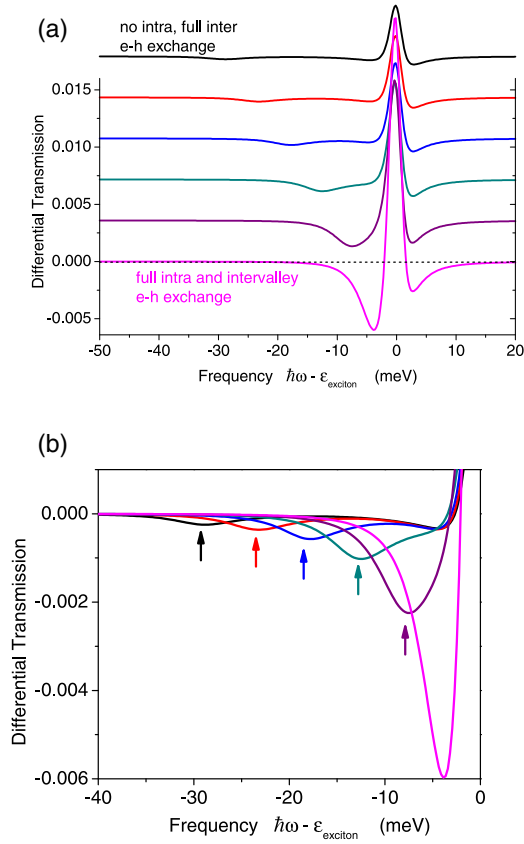
FIG. 7. Differential transmission in the cross-circular configuration ranging from only intervalley exchange to full intravalley and intervalley exchange, \eta_{\text{inter}} = 1 and \eta_{\text{intra}} = 0, 0.2, 0.4, 0.6, 0.8 , and 1 from top to bottom. Except for the bottom curve ( \eta = 1 ), the spectra are shifted vertically for clarity. (b) Same data as in (a) but zoomed in to the biexciton dip, indicated by vertical arrows. The blueshift of the biexciton with increasing intravalley exchange can clearly be seen. The spectra in (b) are not vertically shifted.
