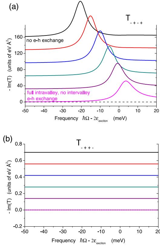
FIG. 3. (a) The two-exciton T -matrix component T_{-++} corresponding to the spectra in Fig. 2. The exchange interaction is varied in the same way as in Fig. 2. The biexciton peak can clearly be seen. (b) Same as (a) but for T_{-+-} . Here, the T -matrix component is zero independent of the e - h exchange strength. The spectra are again shifted vertically for clarity.
