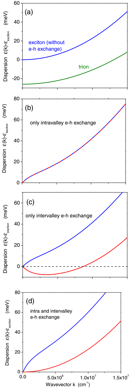
FIG. 1. (a) Exciton (upper curve) and trion (lower curve) dispersion without e -h exchange. (b) Exciton dispersion with intravalley exchange. The two exciton-spin states are degenerate and the two dispersions cannot be distinguished. (c) Exciton dispersion with intervalley exchange; shown are the upper and lower dispersion branches. (d) Exciton dispersion (upper and lower branches) with intravalley and intervalley exchange.
