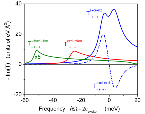
FIG. 12. Comparison of several T -matrix components for the case of Fig. 11. Only results for full exchange strength are shown. In addition to the exciton-exciton and exciton-trion component, the trion-trion component is shown. A peak corresponding to a bound trion-trion complex can clearly be seen at approximately -52 meV. Note that the trion-trion T matrix is small on this scale and has been multiplied by a factor of 5 for better visibility.
