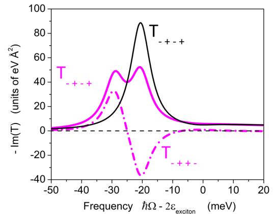
FIG. 6. Same data as in Fig. 5, but only showing the two spectra at full exchange strength (purple curves) and for comparison the curve for zero exchange strength. The split biexciton corresponds to the two dispersion curves shown in Fig. 1(c).
