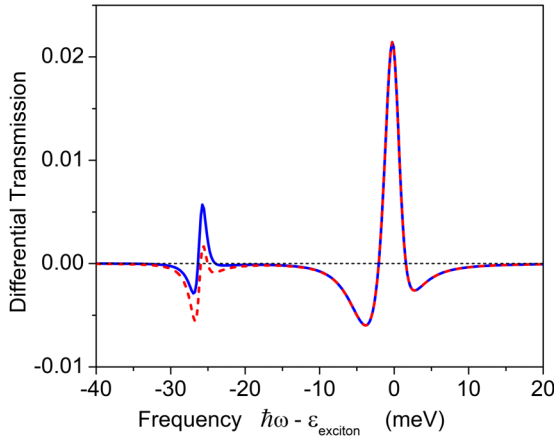
FIG. 13. The effect of pump-induced free-carrier generation on the cross-circular DT. The solid blue curve is the same as in Fig. 10 at full exchange strength, which is without free-carrier generation, and the dashed red curve is with free-carrier generation.
