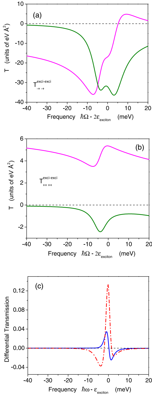
FIG. 9. (a) Real (magenta curve) and imaginary (green curve) part of the two-exciton T -matrix component T_{-+-+} that dominantly determines the DT in the cross-circular configuration. The imaginary part is the same as in Fig. 8. The biexciton resonance is approximately at -3.5 meV. (b) Same as (a) but for T_{++++} . The imaginary part shows a biexciton resonance which is a consequence of the spin coupling due to e -h exchange and is not present without e -h exchange, and the two-exciton continuum that would be present even without e -h exchange. Note that the T matrix in (a) is much larger than in (b). (c) Differential transmission in the cross-circular configuration, dash-dotted red line, which is the same as in Fig. 7, and the co-circular configuration (solid blue line). All results in this figure are at full e -h exchange strength.
