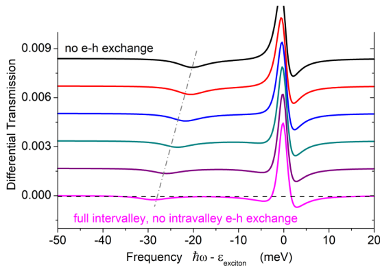
FIG. 4. Differential transmission in the cross-circular configuration without intravalley e - h exchange. The intervalley exchange is increased equidistantly with \eta_{\text{inter}} = 0, 0.2, 0.4, 0.6, 0.8 , and 1 from top to bottom. Except for the bottom curve ( \eta = 1 ), the spectra are shifted vertically for clarity. For clarity, the biexciton resonance is indicated by the dash-dotted line.
