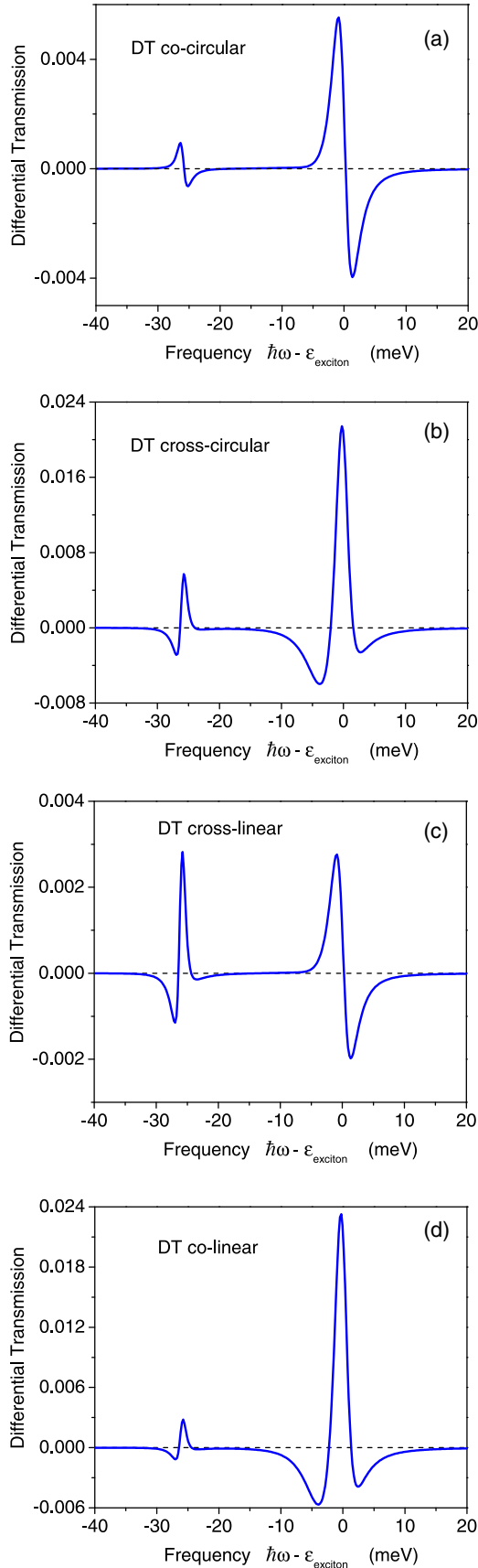
FIG. 14. Differential transmission in the co- and cross-circular and collinear and cross-linear configuration at full intravalley and intervalley exchange.
