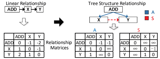
Figure 2: Example of generating position matrices for ancestor-descendent (A) and sibling relationship (S). Position matrix generated from the linear relationship is used in standard Transformers.
