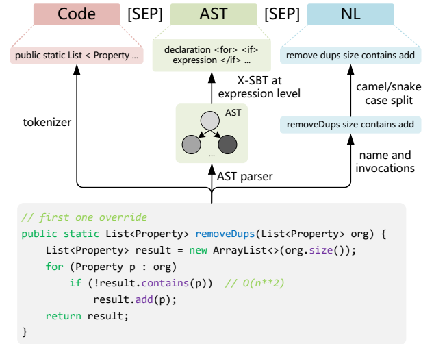
Figure 2: The input of a real world Java code snippet. Due to space constraints, we abbreviated the node names in the AST sequence. “NL” denotes the natural language input.
