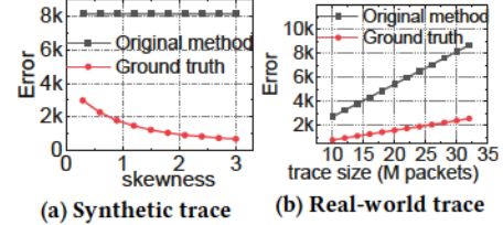
Figure 1: Traditional error bounds are not precise.
