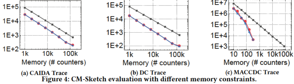
Figure 4: CM-Sketch evaluation with different memory constraints.
