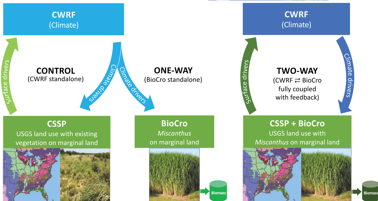
FIGURE 1 Experiment design comparing the control, one-way, and two-way simulations using the climate (CWRf) and crop (BioCro) stand-alone and coupled models. The CWRf has a built-in Conjunctive Surface-Subsurface Process (CSSP) module to incorporate the full surface-atmosphere interaction for climate prediction. The control experiment is the stand-alone CWRf simulation based on USGS' land use categories distributed over the United States, which include the existing natural vegetation on marginal land. The one-way run is the stand-alone BioCro simulation for Miscanthus growth on marginal land as driven by the climate conditions from the control CWRf simulation. The two-way experiment is the fully coupled CWRf-BioCro simulation for growing Miscanthus on marginal land while keeping all others identical to the control experiment. Miscanthus production is estimated by BioCro in the one-way and two-way simulations. The one-way simulation takes the CWRf climate drivers, including precipitation, 2-meter temperature, surface radiation, relative humidity, and wind speed, as the input conditions for Miscanthus to grow on marginal land without feedback onto the climate. The two-way simulation accounts for this feedback, in which the key surface characteristics or drivers for Miscanthus , including leaf area index (LAI), root fraction, albedo, and roughness, differ significantly from the existing vegetation on marginal land and hence are expected to simultaneously alter the regional climate and biomass production. The flow arrow depicts the direction of driving, while different colors distinguish varying state conditions
