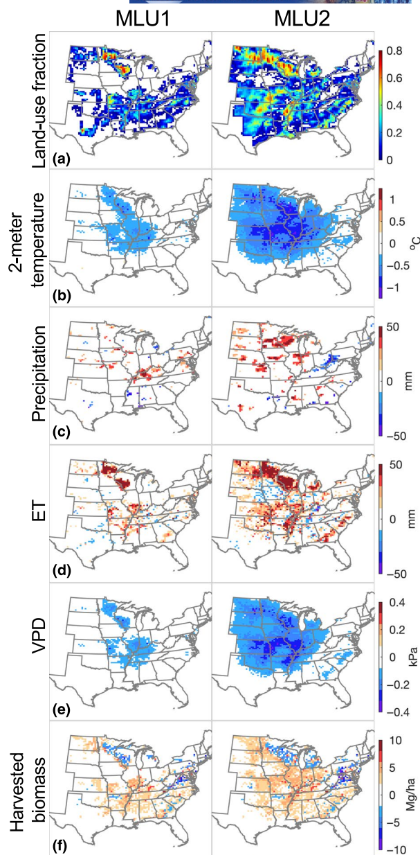
FIGURE 2 Predicted impacts of including the land-atmosphere interactions on the summer climate and the biomass yield for two MLU scenarios. (a) The marginal land fractions based on the CWRf's 30 \times 30 \text{ km}^2 grids for the two MLU scenarios. (b–e) Mean climate differences between the control (i.e., no vegetation change) and presence of Miscanthus on the 43 and 123 Mha of marginal land represented by MLU1 and MLU2, respectively. Climate differences are for the summer (June, July, and August) averaged from 1980 to 2019. This uses the two-way approach which accounts for feedback of climate change on the planted Miscanthus . Climate variables are (b) 2-meter air temperature ( ^{\circ}\text{C} ), (c) precipitation (mm), (d) evapotranspiration (ET, mm), and (e) vapor pressure deficit (VPD, kPa). (f) The difference in Miscanthus stem biomass yield ( \text{Mg ha}^{-1} ) resulting from this climate change by subtracting the one-way (i.e., no feedback) predicted yield from the two-way. All colored grid points passed the t -test at a significance level of 0.05 for the 40-year period
