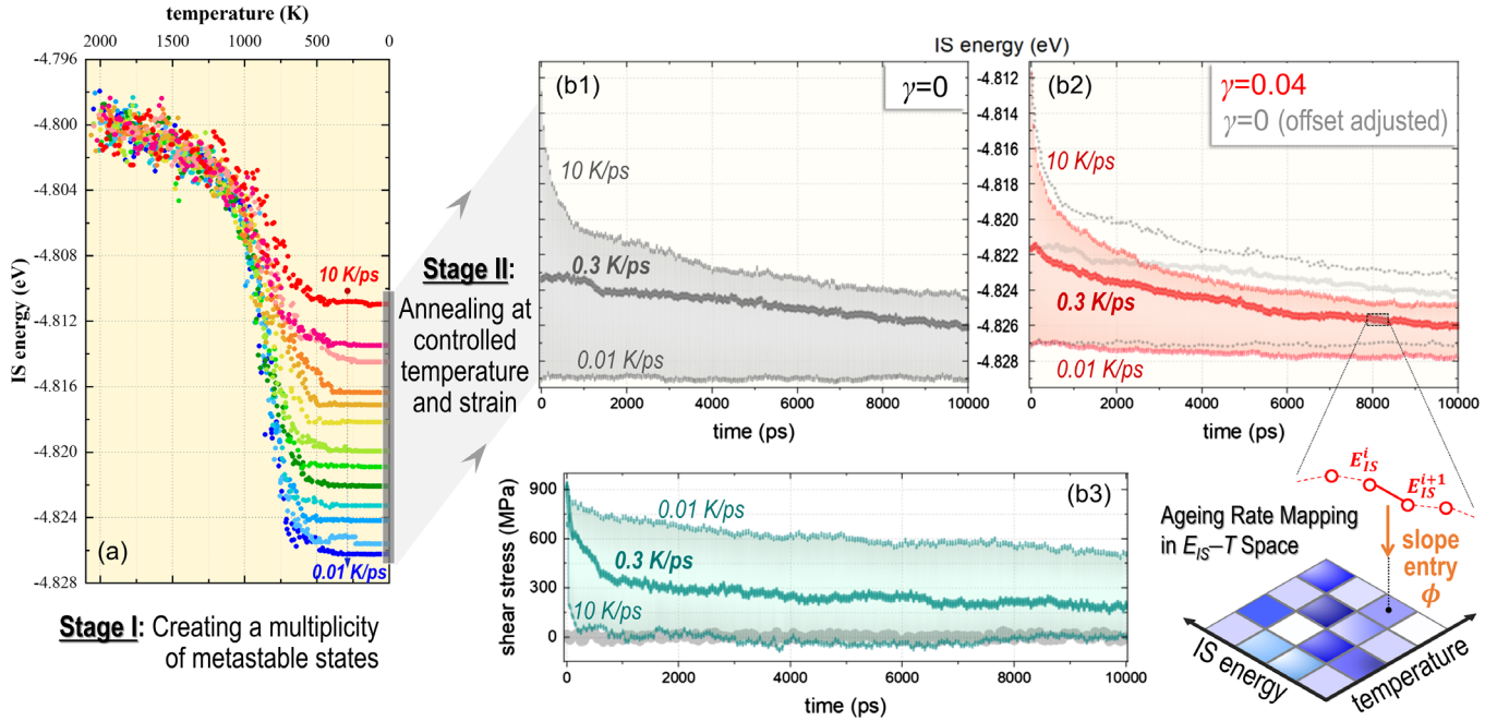
FIG. 1. (a) Glassy samples with various metastability are prepared by cooling at 0.01 \sim 10 \text{ Kps}^{-1} . (b1)–(b2) E_{IS} evolution at 600 K of 0.3 \text{ Kps}^{-1} sample without (gray) and with (red) external shear. (b3) Stress evolution with (green) and without (gray) shear loading. Results at other temperatures are qualitatively similar (Supplemental Material, Fig. S1 [39]).
