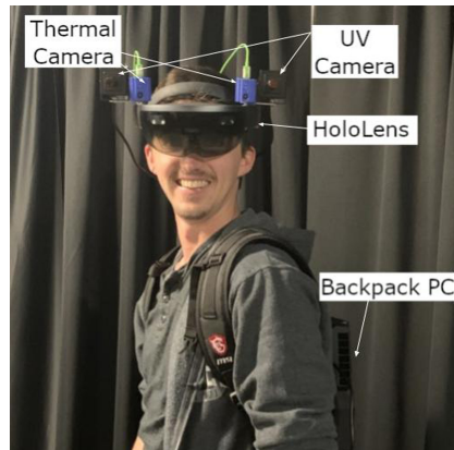
Fig. 2. Annotated photo showing the multi-spectral HoloLens prototype we used in the experiment, including the backpack computer and attached thermal IR and UV cameras.
