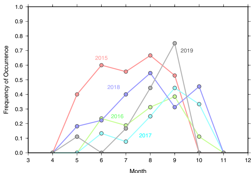
Figure 14. Monthly frequencies of S_{\max} intrusions in profiles from the Shelf Research Fleet from 2015 to 2019. The different years are labeled with different colored symbols.
