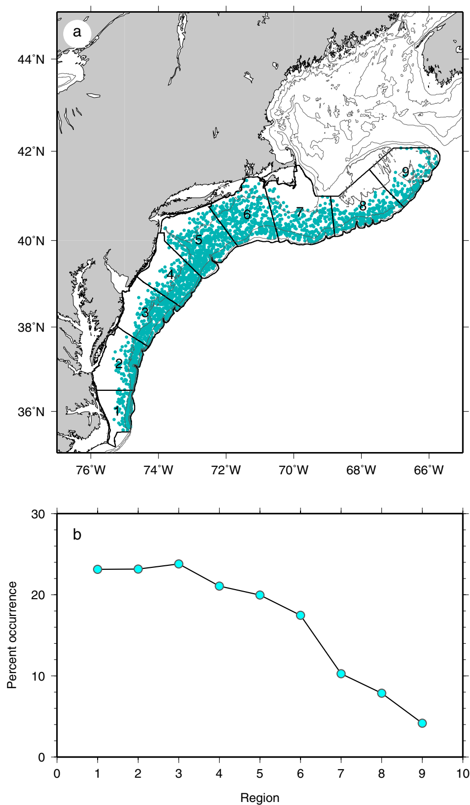
Figure 10. (a) Distribution of S_{\max} intrusions identified in the EcoMon data set between 1990 and 2019 (cyan dots). The 50, 100, and 200 m isobaths are shown in gray. Regional polygons corresponding to Figure 5b are also shown. (b) Percent occurrence of S_{\max} intrusions as identified from the EcoMon data set within each regional polygon shown in Figure 2a.
