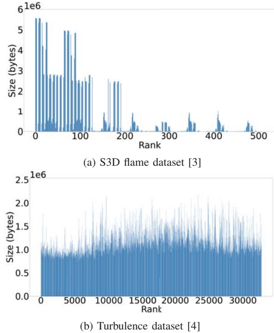
Fig. 1: Size of data held by processes after wavelet transform and ZFP compression for two different datasets demonstrates the imbalanced nature of data distribution. The S3D flame data is spread across 512 processes and the turbulence dataset across 32,768 processes. It can be seen that the degree of imbalance is greater for the S3D (compared to turbulence).
