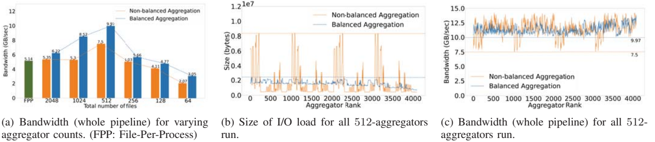
Fig. 8: Results showing the impact of balanced data aggregation for writing S3D flame [3] dataset. (4,096 ranks)
