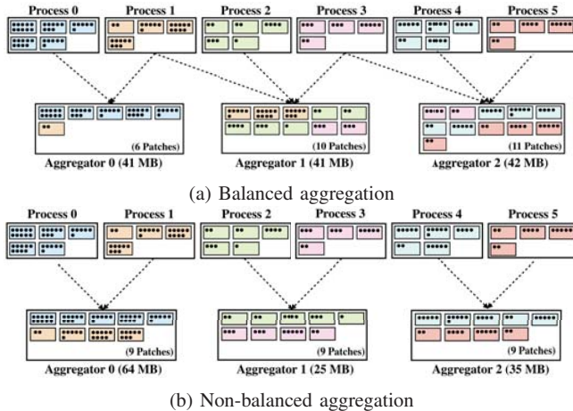
Fig. 5: Our balanced aggregation scheme vs. the non-balanced scheme. Both approaches yield the same number of files (same number of aggregators). However, balanced aggregation generates files of similar size as opposed to the non-balanced scheme where files have varying sizes but the same number of patches. (A filled black circle represents 1M).
