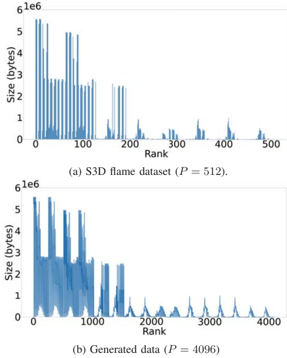
Fig. 10: Micro-benchmark load distributions. The generated data preserves the load distribution patterns in the original data, representing a good candidate for benchmarking at scale.
