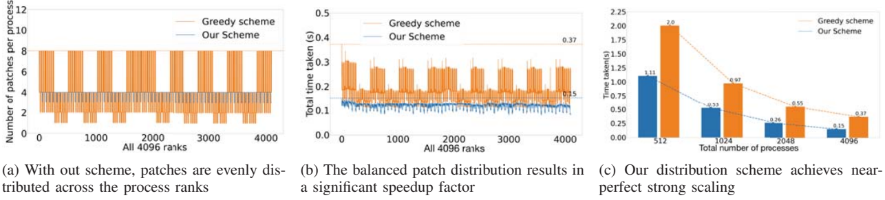
Fig. 6: Compared to the greedy patch distribution scheme, ours reduces the total combined time of the distribution, wavelet transform, and compression steps by more than half. It also exhibits near-perfect strong scaling behavior. (4,096 ranks)
