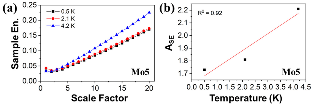
FIG. 3. Results of the RCMSE analysis featuring the (a) sample entropy and (b) the area under the sample entropy curves ( A_{SE} ) for samples tested at 0.5, 2.1, and 4.2 K.
