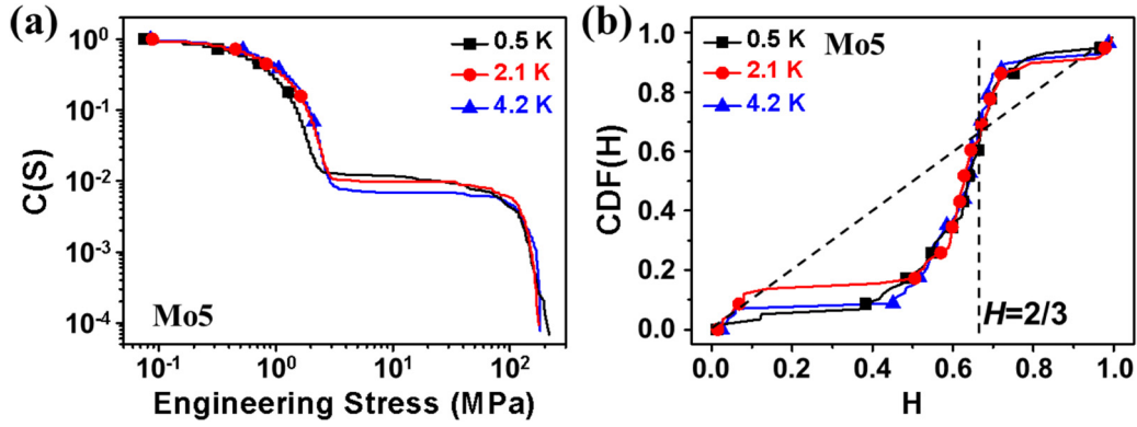
FIG. 2. (a) CCDF, C(S) , of avalanches (engineering stress) observed in the Mo5 alloy during tensile deformation at 0.5, 2.1, and 4.2 K. (b) Cumulative distribution function, CDF(H) , for the large avalanches, with sizes above 100 MPa, with respect to the H values obtained from the Bi test. The black vertical line corresponds to H = 2/3 , and the black oblique line indicates a perfect Poisson process.
