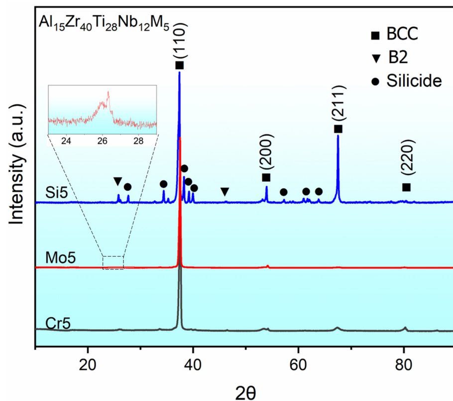
Figure 3. The XRD pattern of the \text{Al}_{15}\text{Zr}_{40}\text{Ti}_{28}\text{Nb}_{12}\text{M}_5 (Cr, Mo, Si) HEAs.
