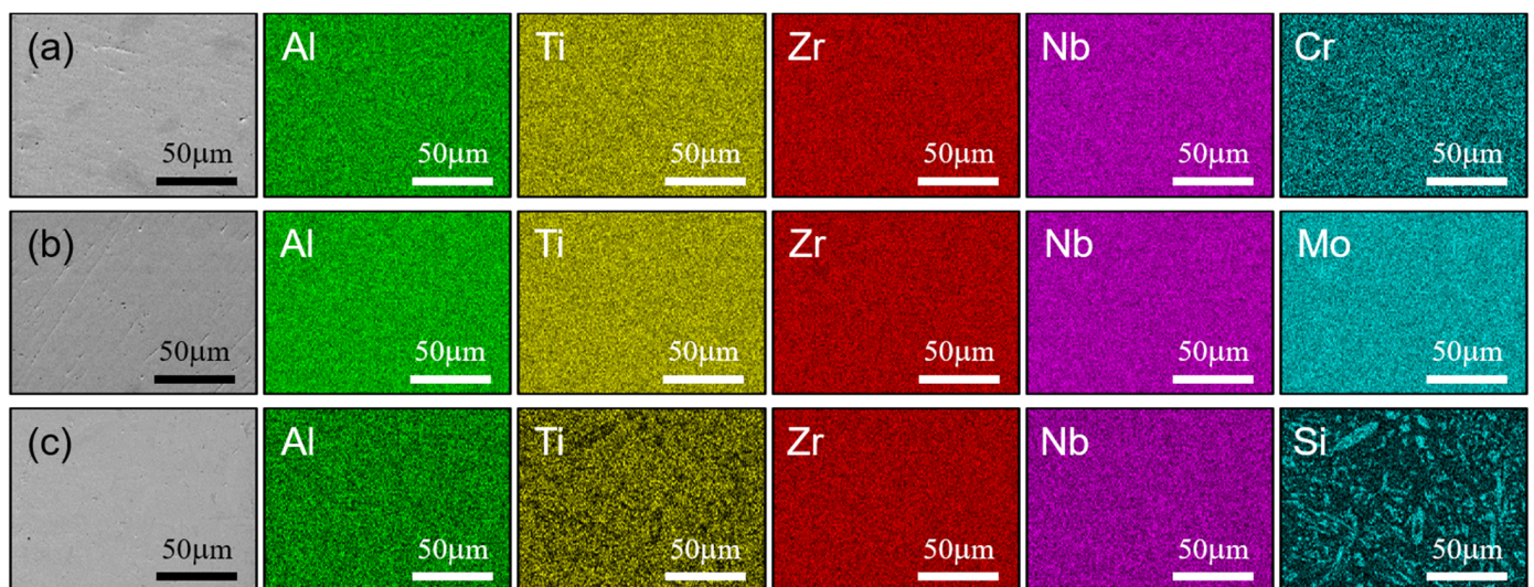
Figure 2. The EDS mappings of the Al 15 Zr 40 Ti 28 Nb 12 M 5 (Cr, Mo, Si) HEAs with secondary electron (SE2). (a) Cr 5 HEA, (b) Mo 5 HEA, and (c) Si 5 HEA.
