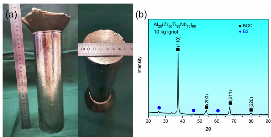
Figure 7. (a) The 10 kg ingot of Al 20 (Zr 50 Ti 35 Nb 15 ) 80 alloy, (b) the XRD pattern of the ingot.
