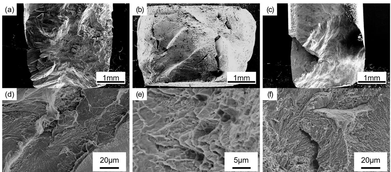
Figure 6. The SEM images of the samples after the compression test and the fracture surface of the Al 15 Zr 40 Ti 28 Nb 12 M 5 (Cr, Mo, Si) HEAs, (a–c) the compressed samples morphology of the Cr 5 , Mo 5 and Si 5 HEAs, respectively; (d–f) the fracture-surface image of the Cr 5 , Mo 5 and Si 5 HEAs, respectively.
