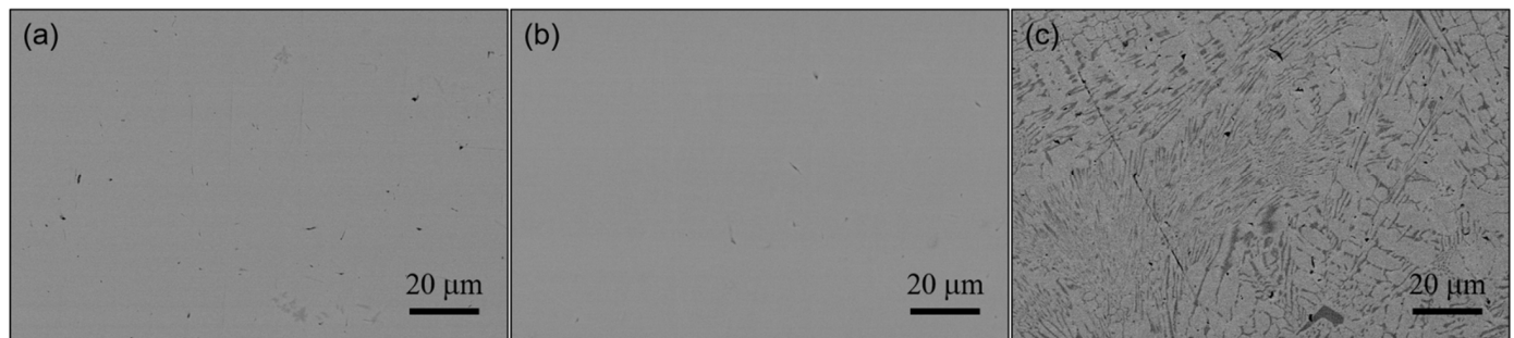
Figure 1. The SEM images of the Al 15 Zr 40 Ti 28 Nb 12 M 5 (Cr, Mo, Si) HEAs with BSE. (a) Cr 5 HEAs, (b) Mo 5 HEAs, and (c) Si 5 HEAs.
