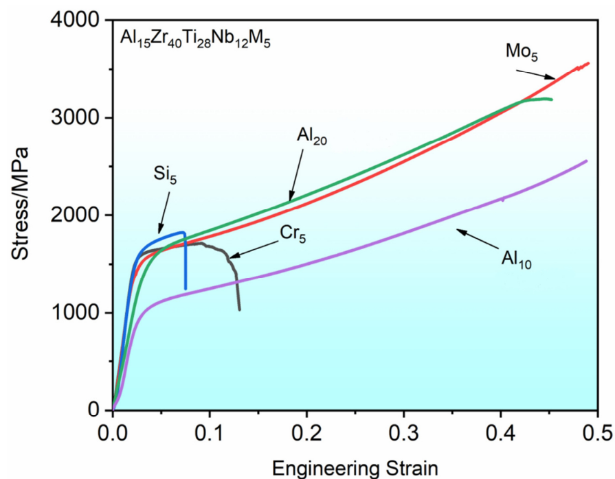
Figure 5. Compressed stress–strain curves of the Al 15 Zr 40 Ti 28 Nb 12 M 5 (Cr, Mo, Si) HEAs and Al x (Zr 50 Ti 35 Nb 15 ) 100−x [15] HEAs (reproduced from Ref. [15], with permission from Elsevier, 2022).
