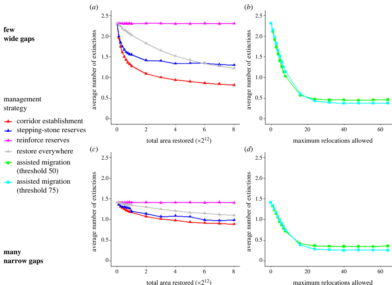
Figure 2. Average number of extinctions after 100 years (y-axis) in climate change simulations, depending on management strategy (colour/shape), amount of area restored for restoration-based modification (a,c) or maximum number of relocations allowed for assisted migration (b,d; x-axis), and environment structure (a,b: few wide gaps, c,d: many narrow gaps). Each point is the mean of 10 000 simulations.
