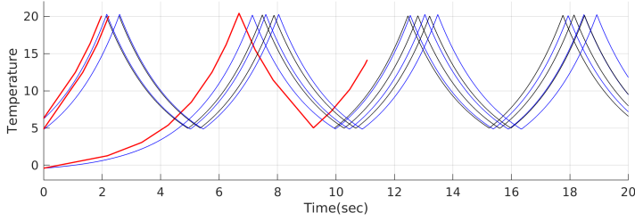
Fig. 15. Comparison of hybrid automaton learned by our method and the membership-based method. The black traces are from the original system, the blue traces are from the system learned by our method. While the red traces are from the system learned by the membership-based method.
