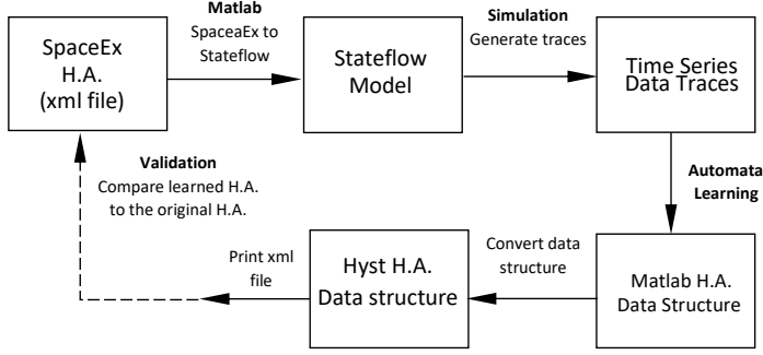
Fig. 2. Overview of the validation of the proposed framework for the method described in this paper. A given hybrid automaton is specified in the SpaceEx/HyST [7, 20] format, automatically translated to a Simulink/Stateflow model using HyST [6, 7], simulated to generate time series data (traces). The hybrid automata learning framework is then applied to these traces, and a learned hybrid automaton is generated in the SpaceEx/HyST format, and simulated again to generate traces to validate the learned model's behaviors against the original model's behaviors.
