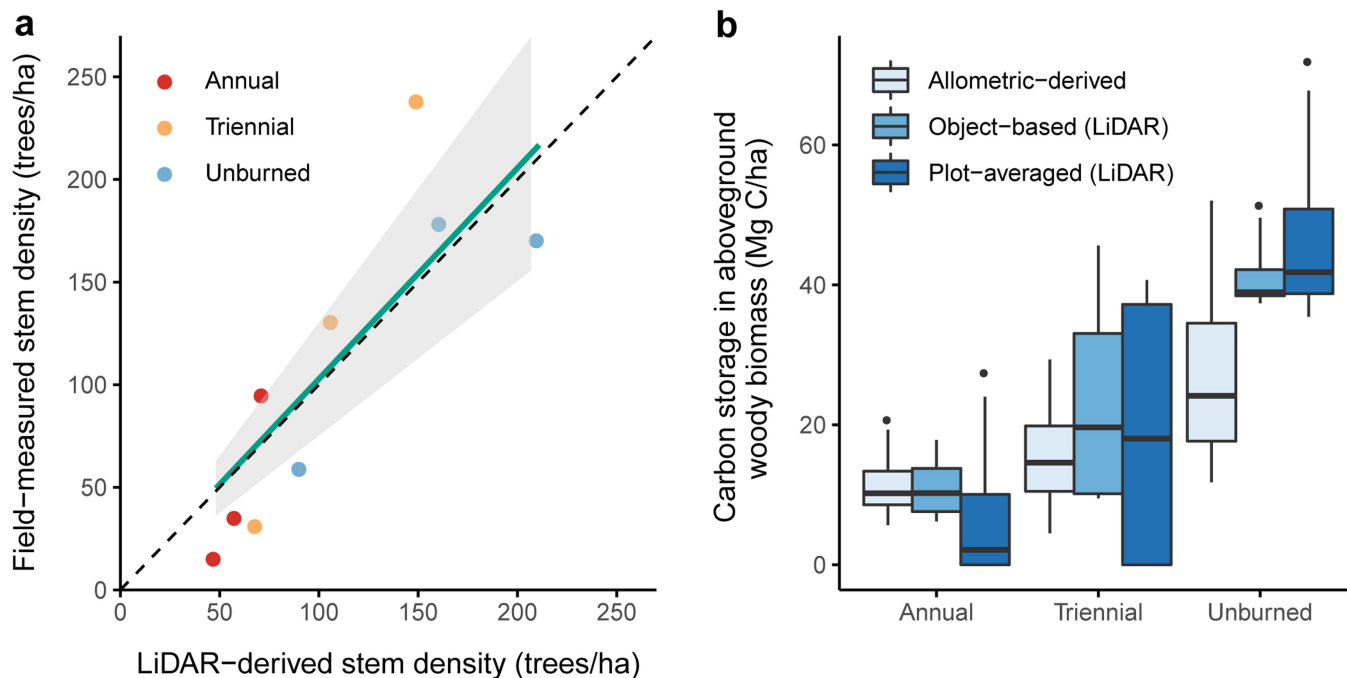
Extended Data Fig. 8 | The validation of the object-based method to estimate aboveground woody biomass. a , The correlation between LiDAR-derived stem density for trees with height > 5m (trees ha -1 ) and field-measured stem density (trees ha -1 ). The field-measured stem density was from ref. 52 , which surveyed tree heights in eight 10-m-radius plots at each annual, triennial and unburned treatment in Kambeni, Numbi and Shabeni strings at the Pretoriuskop landscape in Kruger National Park, South Africa. The regression line indicates the significant linear fit and the shaded bands illustrate the 95% confidence interval of the linear fit. The dashed line indicates the 1:1 line. b , Differences in aboveground woody biomass between allometric-derived, object-based and plot-averaged estimates. The
