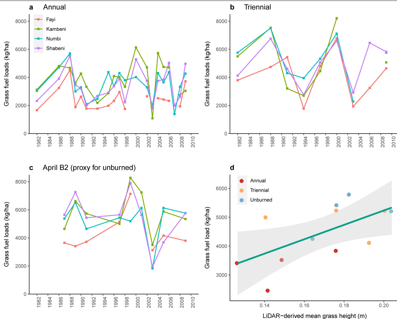
Extended Data Fig. 4 | Long-term monitoring of grass fuel loads and their correlation to LiDAR-derived mean grass height. a–c , Grass fuel loads ( \text{kg ha}^{-1} ) for annual ( a ), triennial ( b ) and April B2 (that is, burning in April for every two years, as a proxy for unburned) ( c ) treatments from 1982 to 2009 for different strings at the Pretoriuskop landscape in Kruger National Park, South Africa. Disconnected lines indicate missing data for specific years. d , The correlation between averaged grass fuel loads from 1982 to 2009 and
