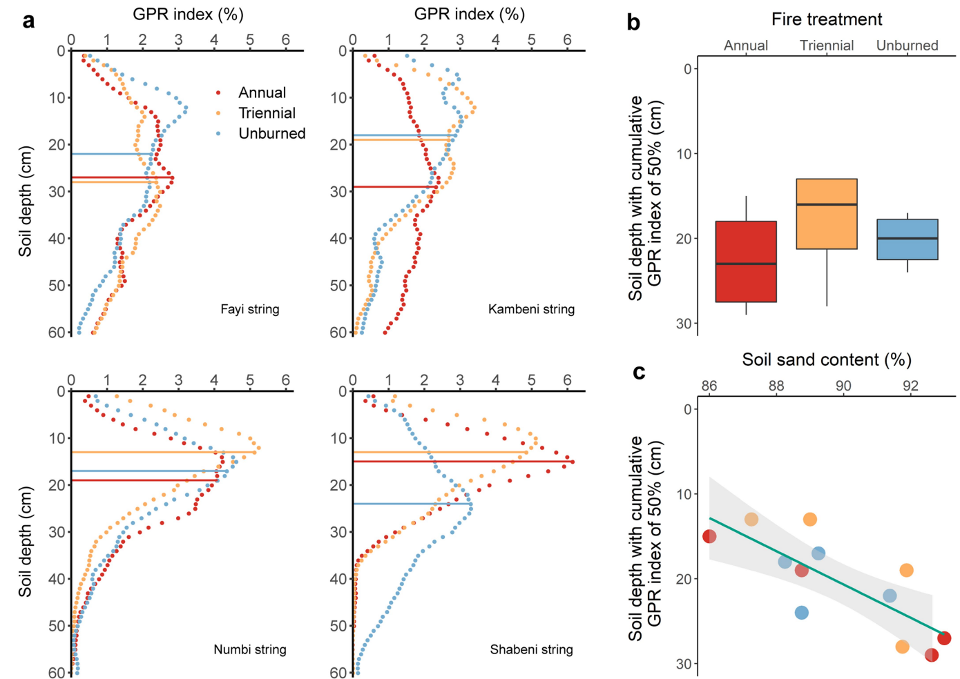
Extended Data Fig. 6 | Depth distribution of coarse-lateral-root biomass across fire treatments and soil sand content. a , Depth distribution of the GPR index (% in the number of pixels above the threshold for root detections) as an indicator of coarse-lateral-root biomass allocation throughout the soil column across different fire treatments at each string. Horizontal lines indicate the depth (cm) at which the GPR index reaches 50% of the total detections in the 60-cm soil column. b , Effects of fire treatment on the depth distribution of
