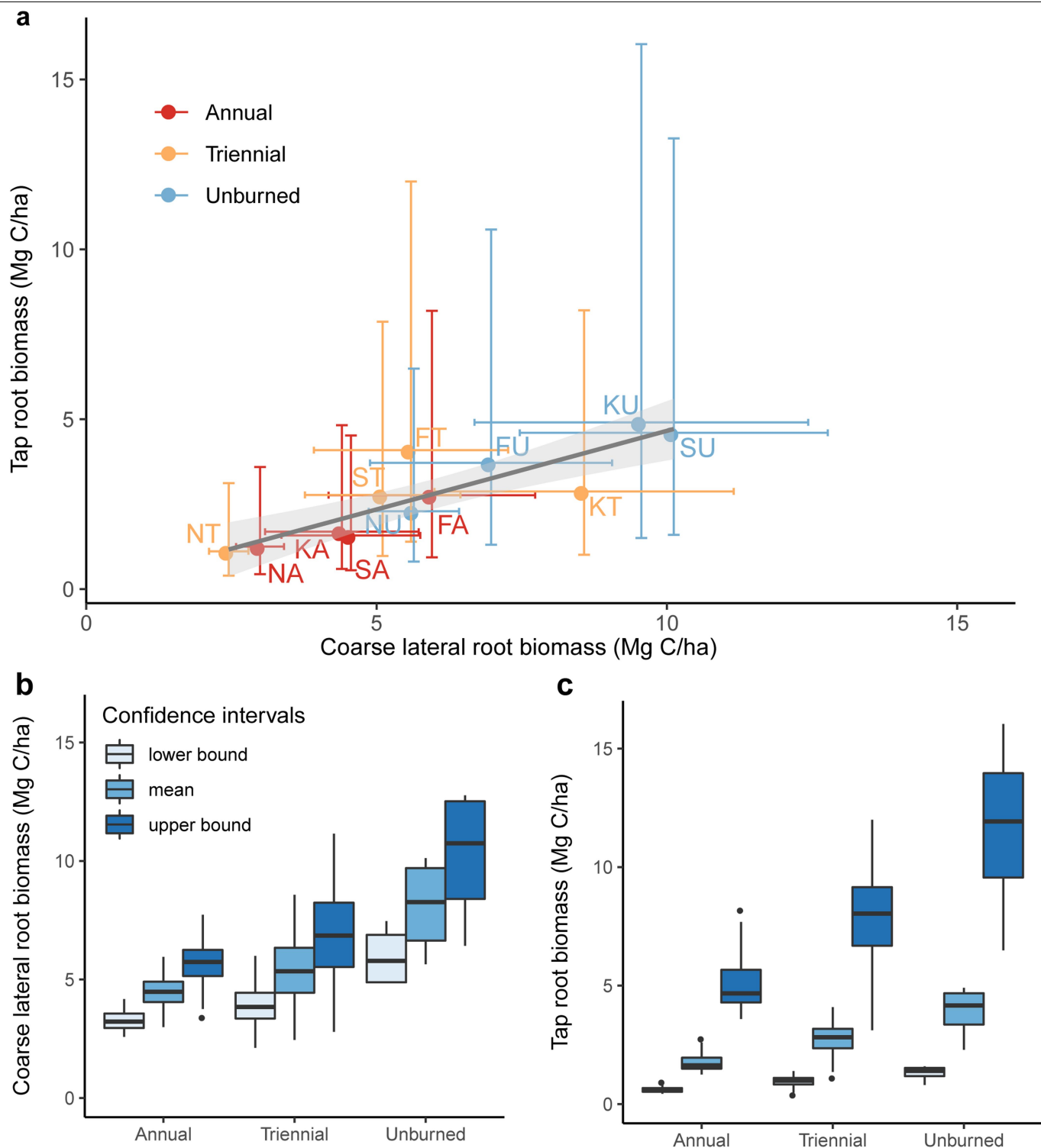
Extended Data Fig. 5 | The uncertainty of coarse lateral and taproot biomass estimates. a , The uncertainty of coarse lateral and taproot biomass for each treatment replicate. Error bars indicate the 95% confidence interval for coarse lateral and taproot biomass estimates derived from fitting regression lines (see Supplementary Figs. 5 and 10). Coarse-lateral-root biomass estimates were significantly correlated with taproot biomass estimates ( R^2 = 0.75 , P < 0.001 ). Letters F, K, N and S indicate Fayi, Kambeni,
