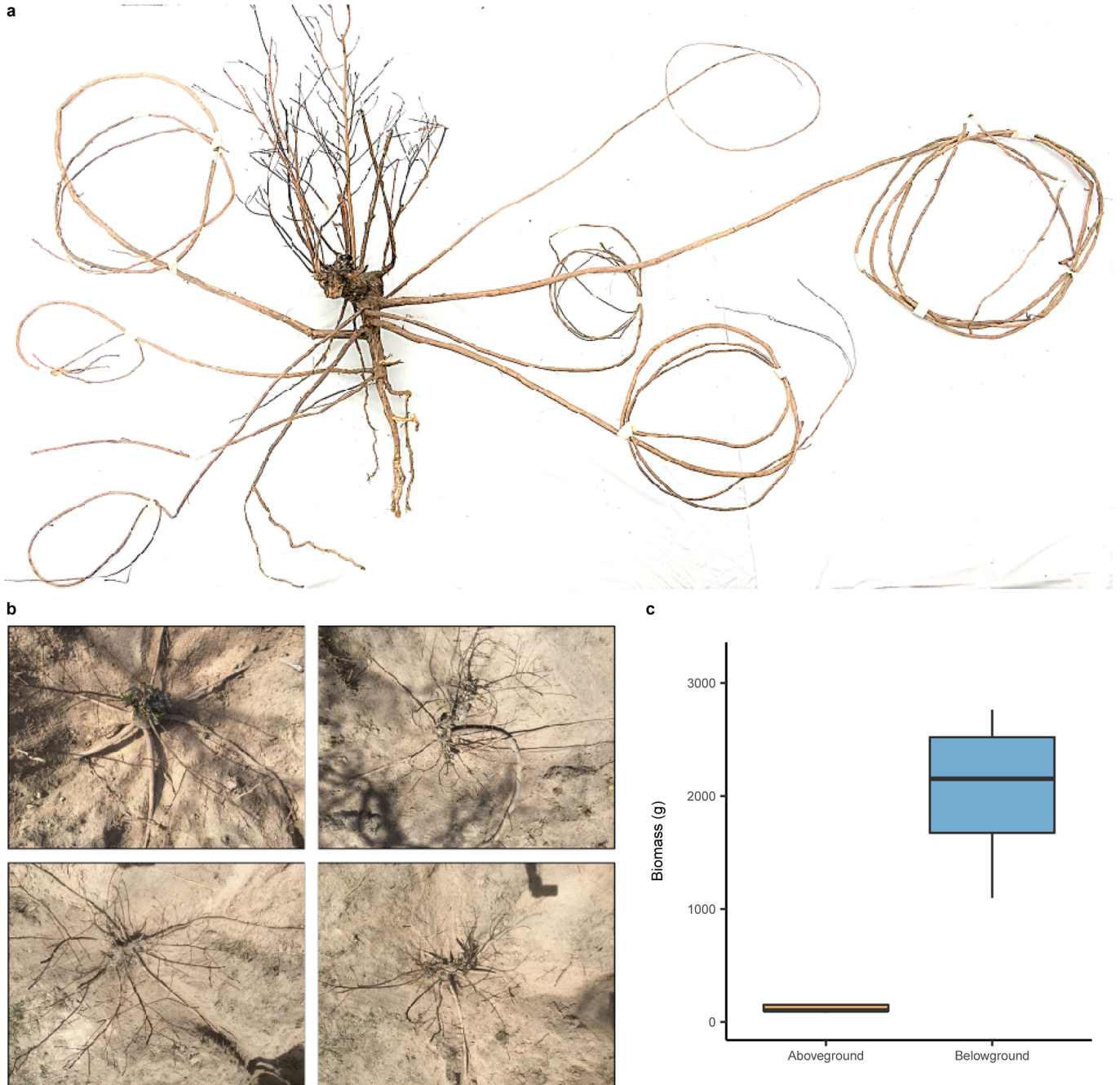
Extended Data Fig. 1 | An example showing belowground to aboveground biomass allocation for resprouting Terminalia sericea . a, b, Five T. sericea individuals that have experienced annual burning were excavated in the Pretoriuskop landscape in Kruger National Park, South Africa. c, The difference
