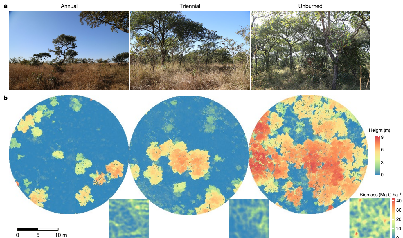
Fig. 1 | Vegetation characteristics of experimental burn plots in a mesic savanna in Kruger National Park, South Africa. a , Example pictures showing vegetation structure in different fire treatments. b , Examples of tree canopy cover and height (that is, 30-m-diameter circular plots) derived from airborne light detection and ranging and belowground coarse-root biomass (that is,
