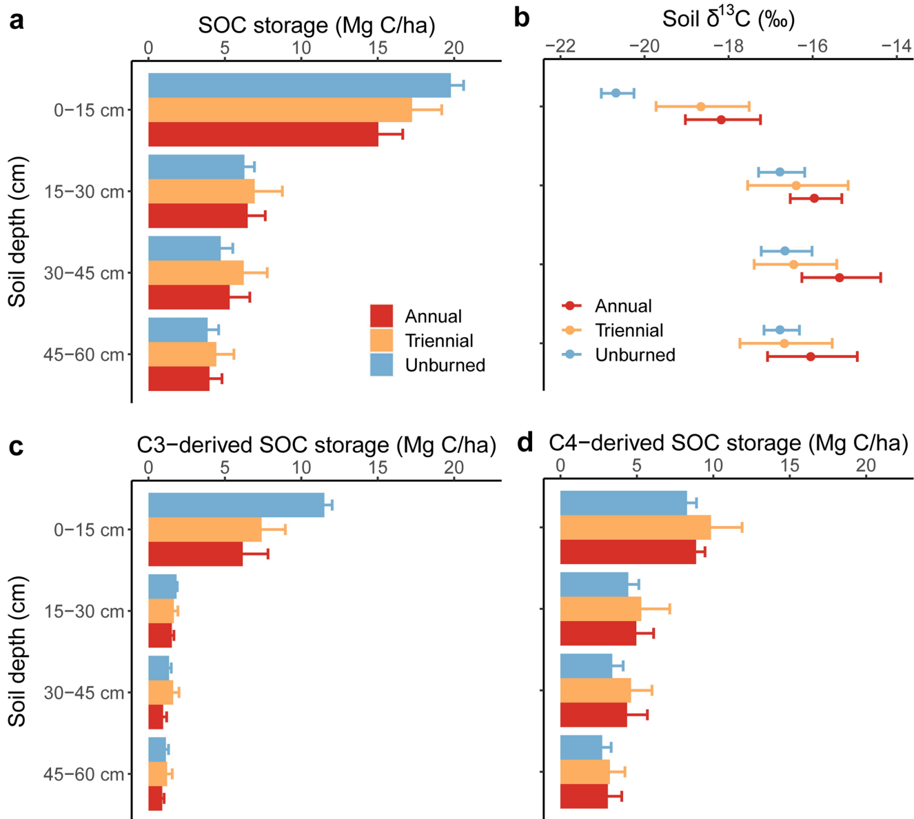
Extended Data Fig. 3 | Changes in SOC storage and soil \delta^{13}\text{C} across different fire treatments throughout the 60-cm soil column. Effects of fire treatments on total SOC storage ( \text{Mg C ha}^{-1} ) (a), soil \delta^{13}\text{C} (‰) (b), C 3 -derived SOC storage
