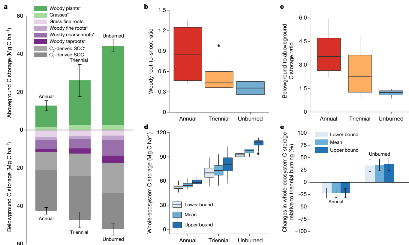
Fig. 2 | Changes in whole-ecosystem carbon storage across fire treatments.
